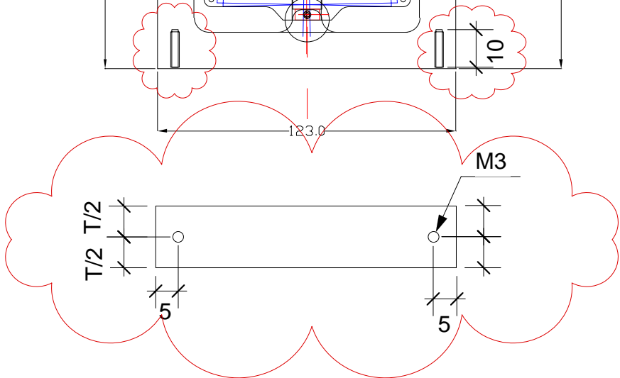
M3 screw holes for module holding
