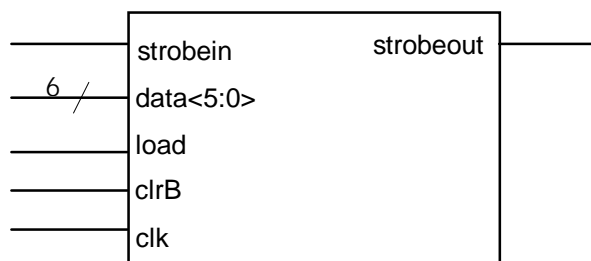
Figure 3.11. Strobe Delay Register Inputs/Outputs.
