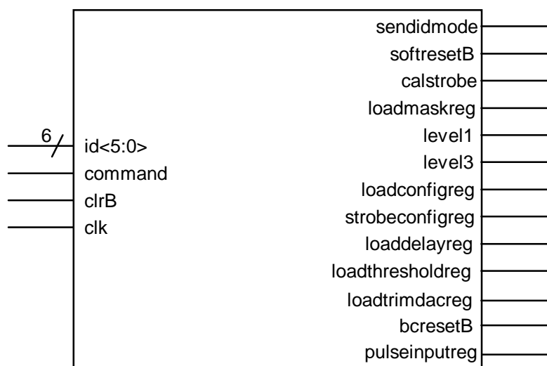
Figure 3.9B. Command Decoder Inputs/Outputs (ABCD2T).
