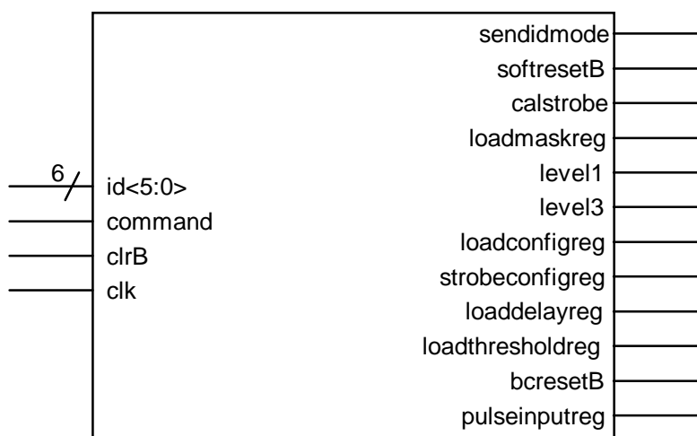
Figure 3.9A. Command Decoder Inputs/Outputs (ABCD2NT).
