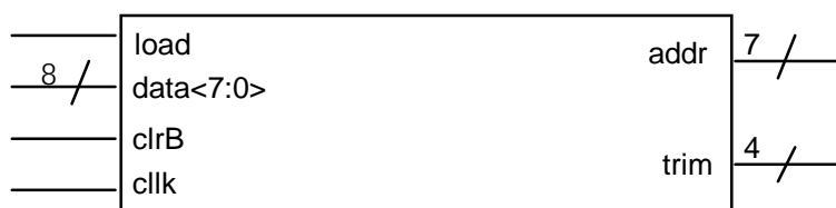
Figure 3.13A. Trim DAC Register Inputs/Outputs.
