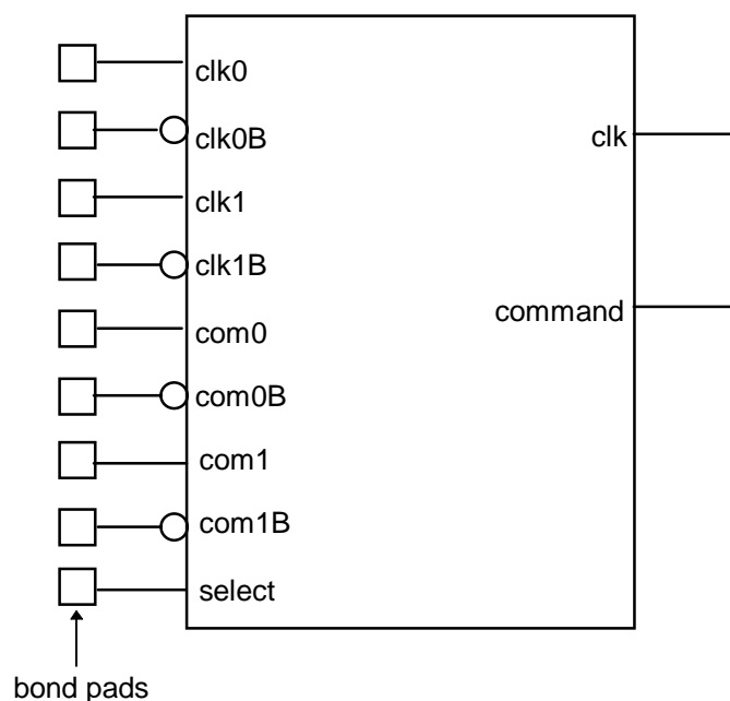
Figure 3.14. Clock &amp; Command Data Inputs.
