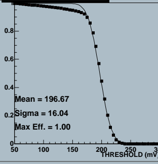
Efficiency, chip 4
