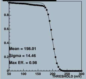
Efficiency, chip 3
