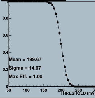
Efficiency, chip 4
