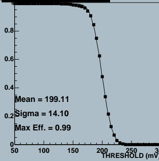
Efficiency, chip 2
