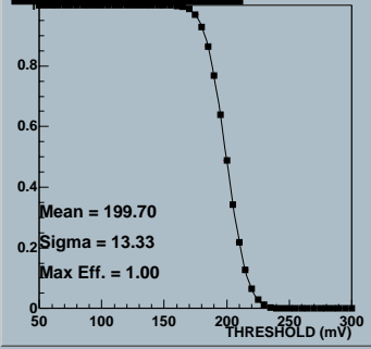
Efficiency, chip 5
