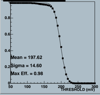
Efficiency, chip 5
