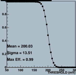
Efficiency, chip 2
