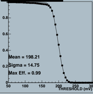
Efficiency, chip 4
