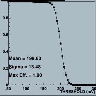
Efficiency, chip 4
