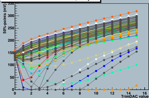
TrimDAC characteristics, chip 10
