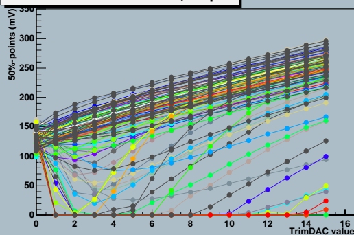
TrimDAC characteristics, chip 9
