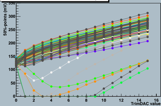
TrimDAC characteristics, chip 4
