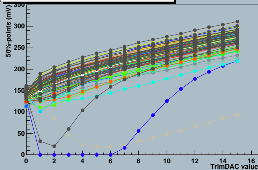
TrimDAC characteristics, chip 5
