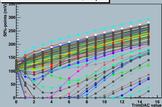
TrimDAC characteristics, chip 8
