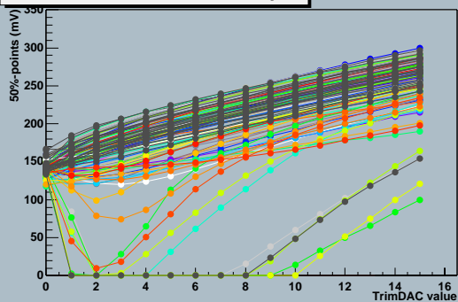
TrimDAC characteristics, chip 2
