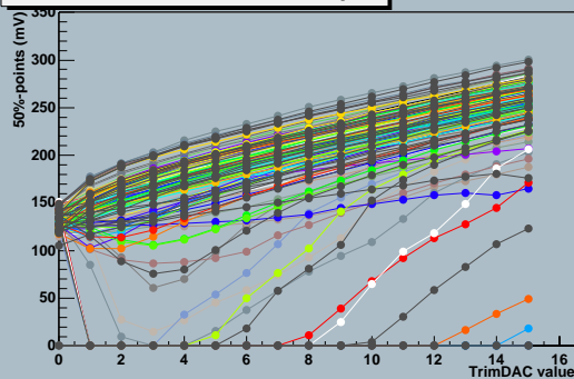
TrimDAC characteristics, chip 3
