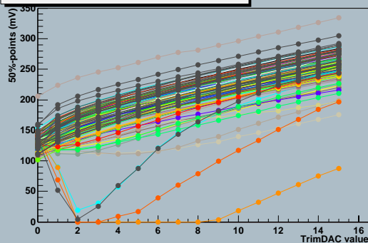
TrimDAC characteristics, chip 11
