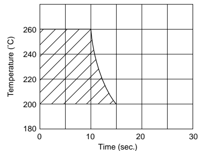
Allowable Flow Soldering Temperature and Time
