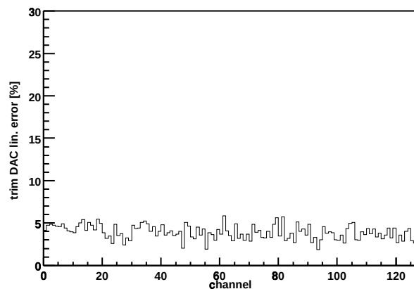
Chip Z36459A-W03-X01-Y07 trim DAC lin. error
