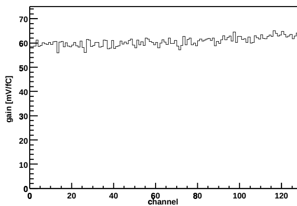
Chip Z36459A-W03-X01-Y07 Gain vs. channel
