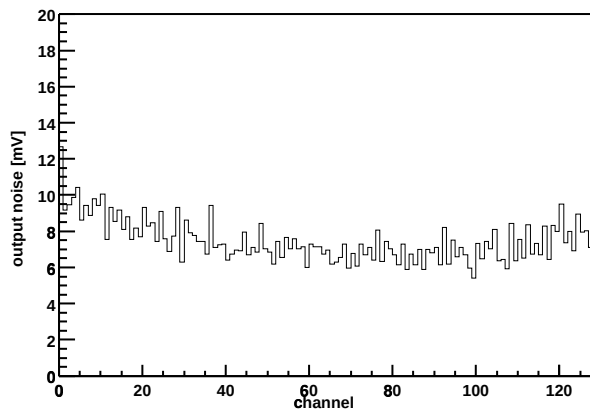
Chip Z36459A-W03-X01-Y07 Output noise vs. channel
