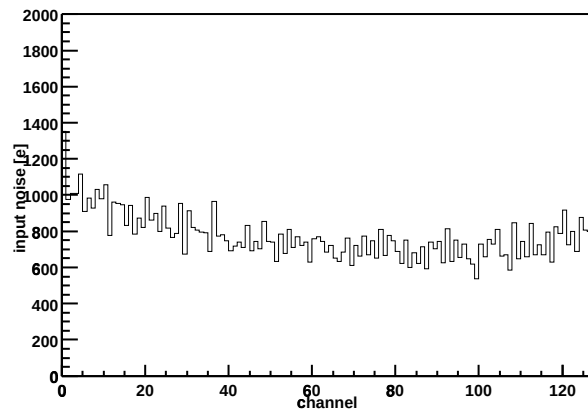
Chip Z36459A-W03-X01-Y07 Input noise vs. channel
