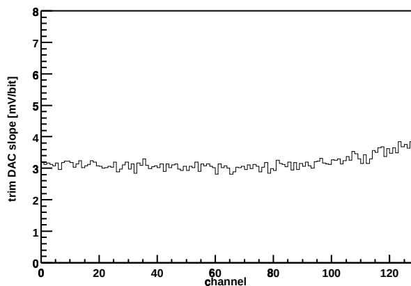
Chip Z36459A-W03-X01-Y07 Trim DAC slope vs. channel
