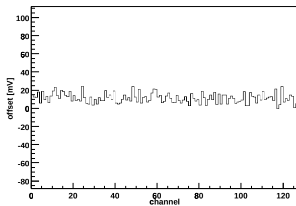
Chip Z36459A-W03-X01-Y07 Offset vs. channel
