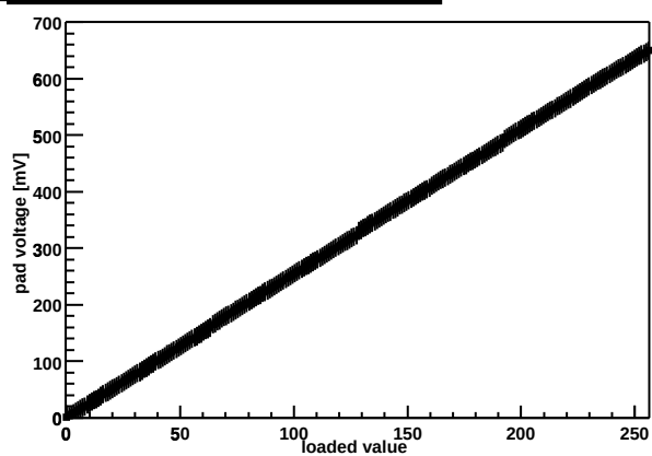
Chip Z36459A-W03-X01-Y07 threshold DAC
