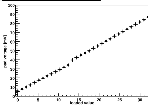
Chip Z36459A-W03-X01-Y07 preamp DAC
