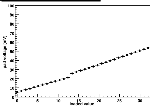
Chip Z36459A-W03-X01-Y07 shaper DAC
