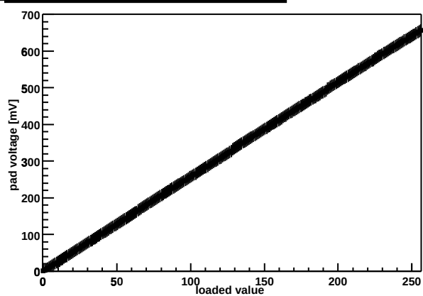
Chip Z36459A-W03-X01-Y08 threshold DAC
