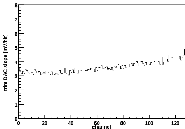
Chip Z36459A-W03-X01-Y08 Trim DAC slope vs. channel
