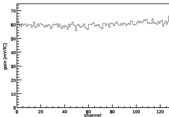
Chip Z36459A-W03-X01-Y08 Gain vs. channel
