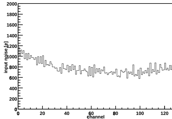
Chip Z36459A-W03-X01-Y08 Input noise vs. channel
