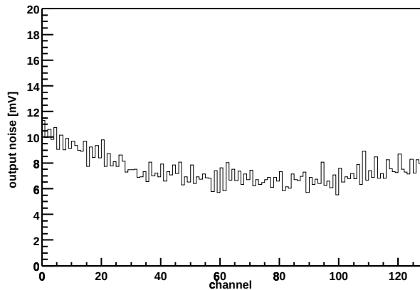
Chip Z36459A-W03-X01-Y08 Output noise vs. channel
