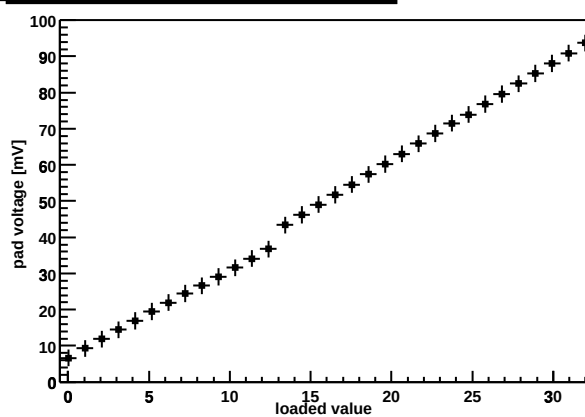
Chip Z36459A-W03-X01-Y08 preamp DAC
