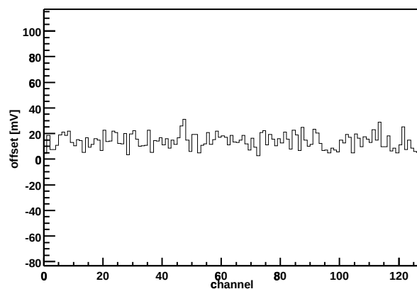
Chip Z36459A-W03-X01-Y08 Offset vs. channel
