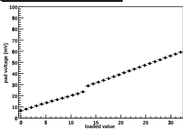
Chip Z36459A-W03-X01-Y08 shaper DAC
