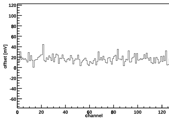
Chip Z36459A-W03-X01-Y10 Offset vs. channel
