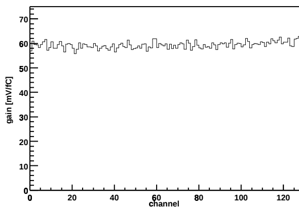
Chip Z36459A-W03-X01-Y10 Gain vs. channel
