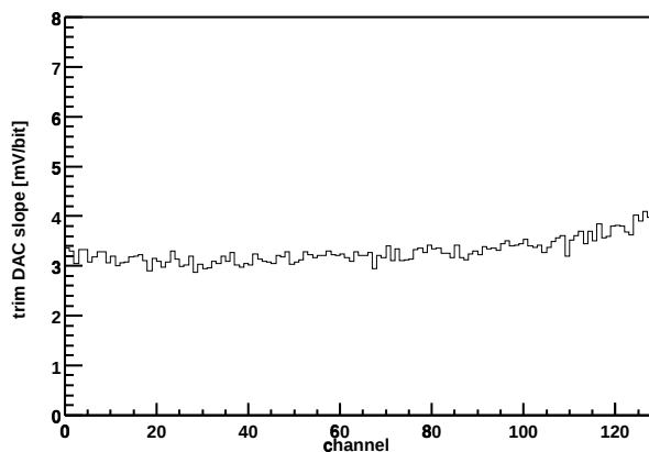
Chip Z36459A-W03-X01-Y10 Trim DAC slope vs. channel
