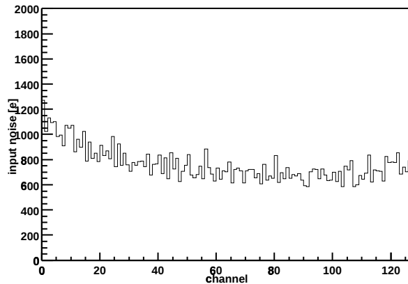
Chip Z36459A-W03-X01-Y10 Input noise vs. channel
