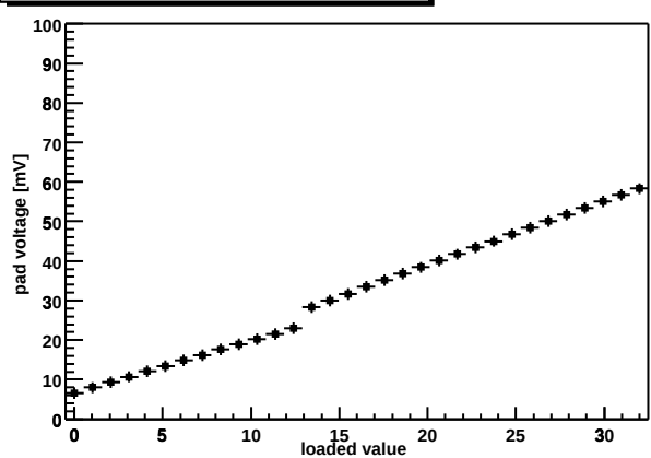
Chip Z36459A-W03-X01-Y10 shaper DAC
