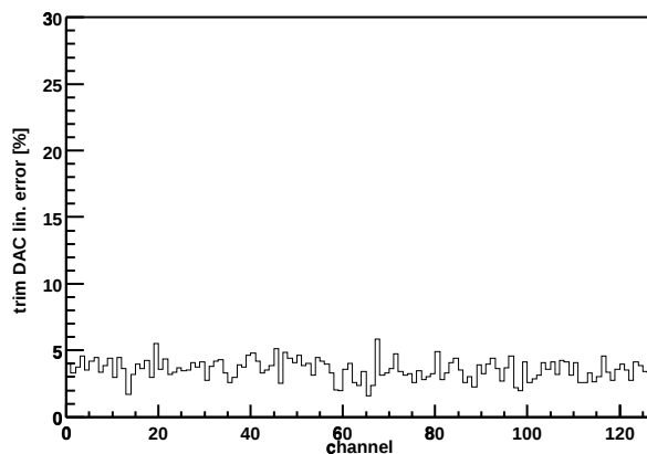
Chip Z36459A-W03-X01-Y10 trim DAC lin. error
