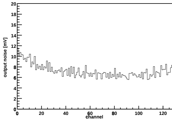
Chip Z36459A-W03-X01-Y10 Output noise vs. channel
