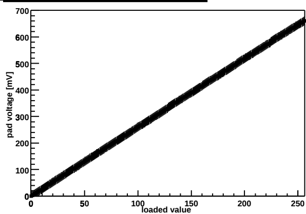
Chip Z36459A-W03-X01-Y10 threshold DAC
