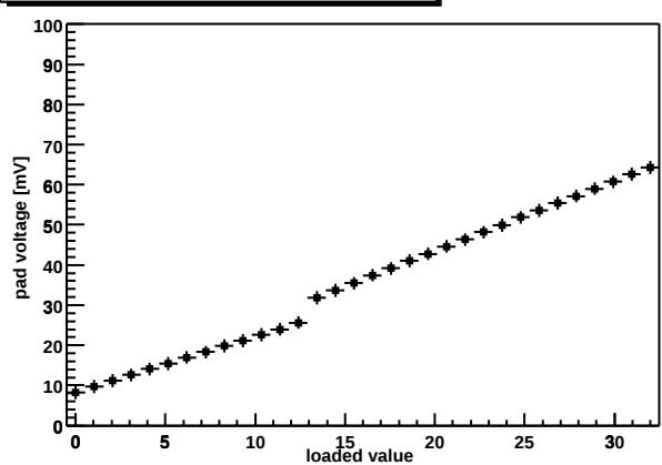
Chip Z36459A-W03-X01-Y11 shaper DAC
