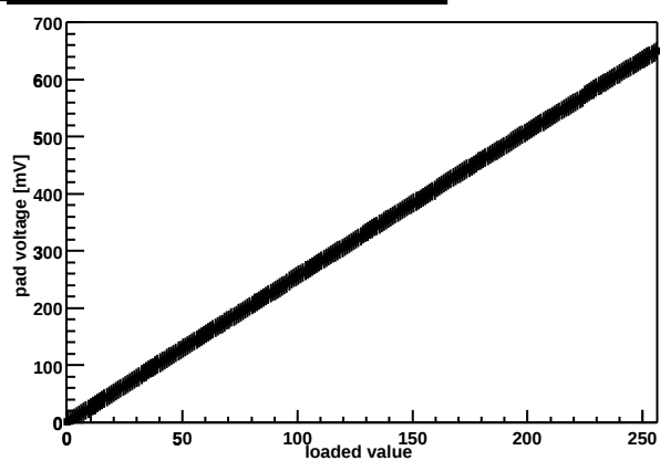
Chip Z36459A-W03-X01-Y11 threshold DAC
