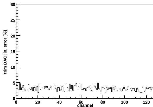
Chip Z36459A-W03-X01-Y11 trim DAC lin. error
