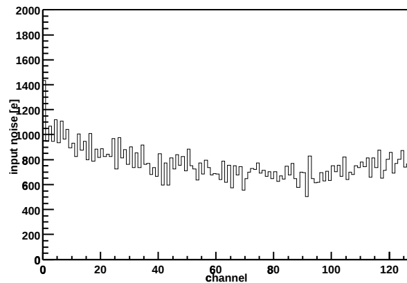
Chip Z36459A-W03-X01-Y11 Input noise vs. channel
