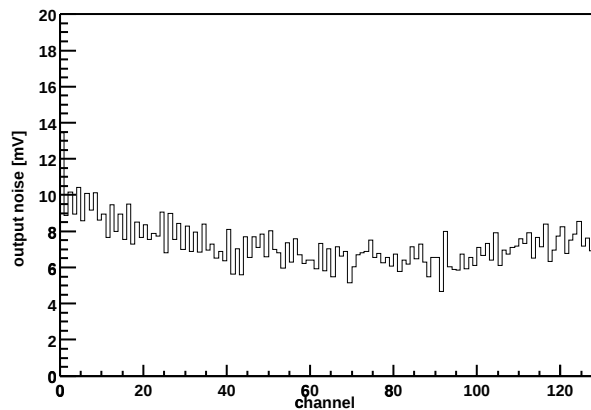
Chip Z36459A-W03-X01-Y11 Output noise vs. channel
