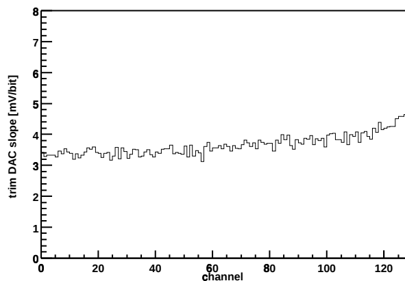
Chip Z36459A-W03-X01-Y11 Trim DAC slope vs. channel
