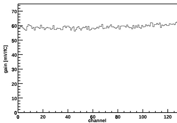
Chip Z36459A-W03-X01-Y11 Gain vs. channel
