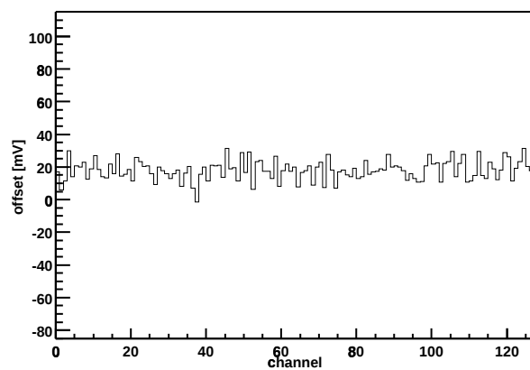
Chip Z36459A-W03-X01-Y11 Offset vs. channel
