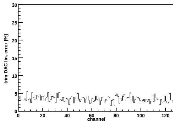
Chip Z36459A-W03-X01-Y12 trim DAC lin. error
