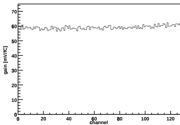
Chip Z36459A-W03-X01-Y12 Gain vs. channel
