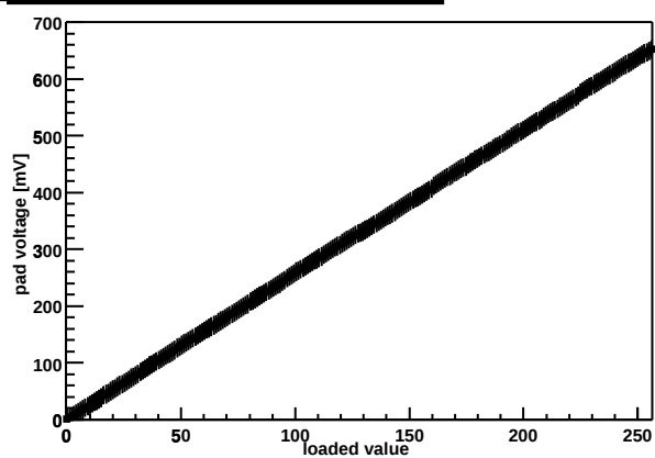
Chip Z36459A-W03-X01-Y12 threshold DAC
