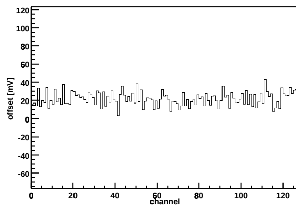
Chip Z36459A-W03-X01-Y12 Offset vs. channel
