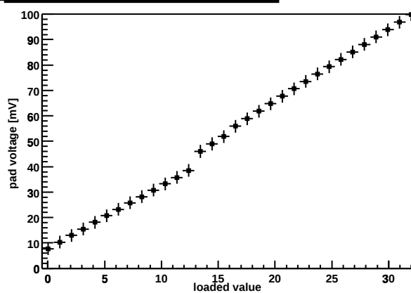
Chip Z36459A-W03-X01-Y12 preamp DAC
