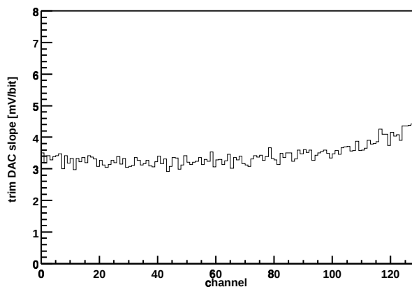
Chip Z36459A-W03-X01-Y12 Trim DAC slope vs. channel
