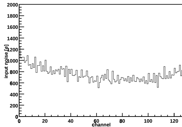
Chip Z36459A-W03-X01-Y12 Input noise vs. channel
