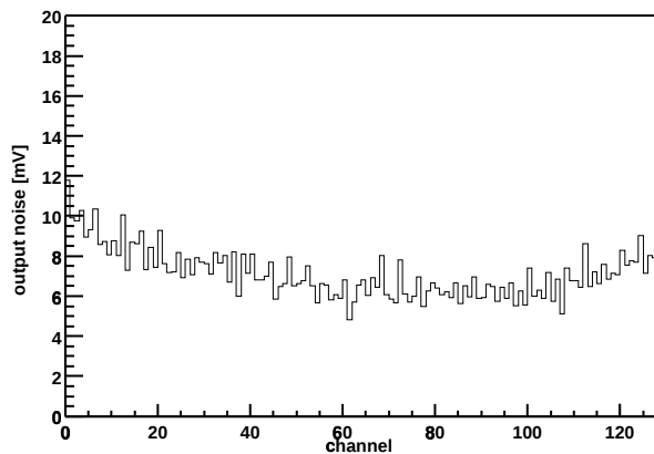
Chip Z36459A-W03-X01-Y12 Output noise vs. channel
