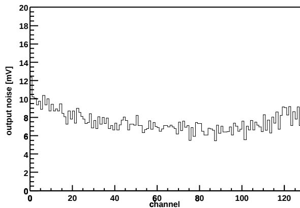
Chip Z36459A-W03-X02-Y06 Output noise vs. channel
