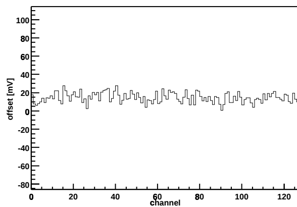
Chip Z36459A-W03-X02-Y06 Offset vs. channel
