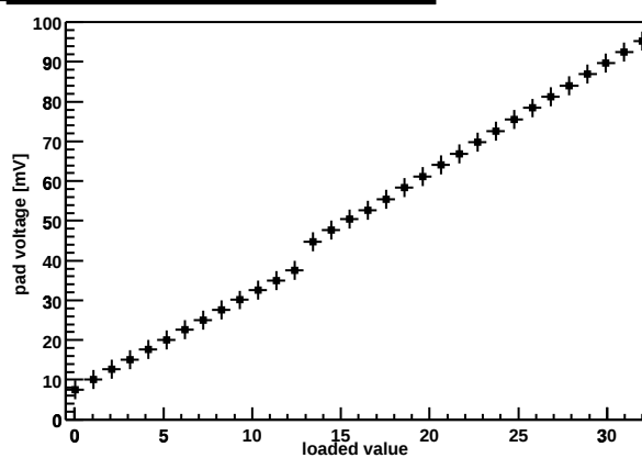
Chip Z36459A-W03-X02-Y06 preamp DAC
