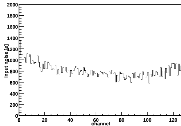
Chip Z36459A-W03-X02-Y06 Input noise vs. channel
