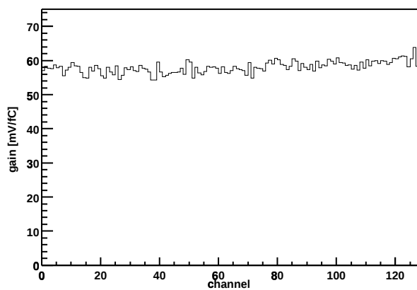
Chip Z36459A-W03-X02-Y06 Gain vs. channel
