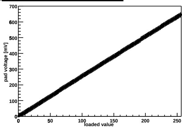
Chip Z36459A-W03-X02-Y06 threshold DAC
