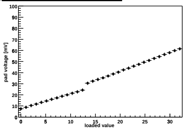
Chip Z36459A-W03-X02-Y06 shaper DAC
