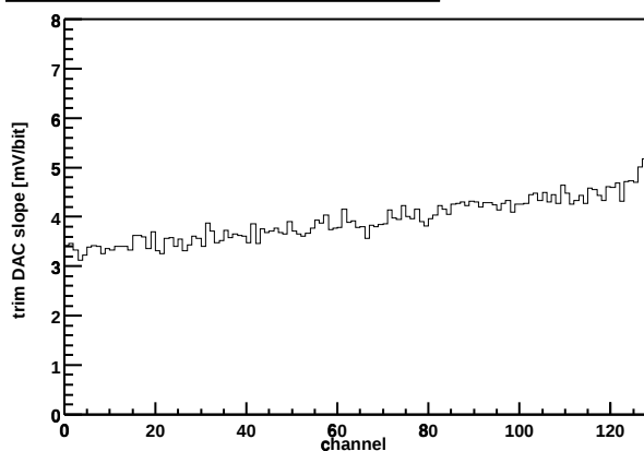
Chip Z36459A-W03-X02-Y06 Trim DAC slope vs. channel
