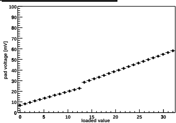
Chip Z36459A-W03-X02-Y10 shaper DAC
