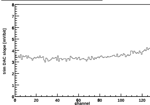
Chip Z36459A-W03-X02-Y10 Trim DAC slope vs. channel
