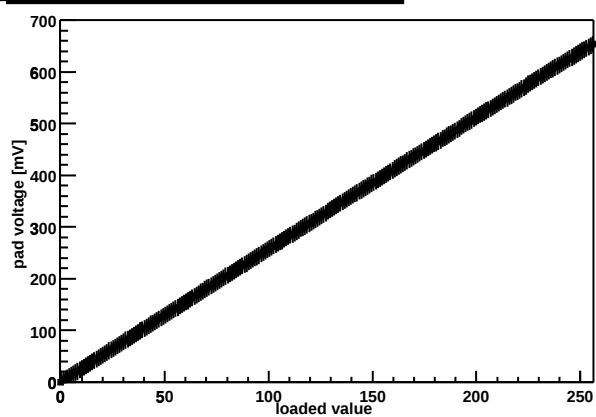
Chip Z36459A-W03-X02-Y10 threshold DAC
