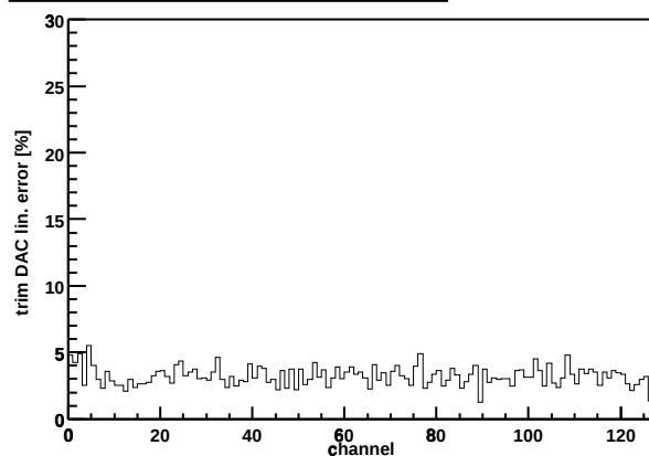
Chip Z36459A-W03-X02-Y10 trim DAC lin. error
