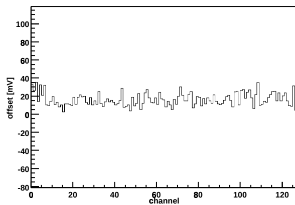
Chip Z36459A-W03-X02-Y10 Offset vs. channel
