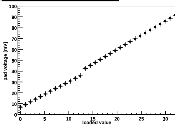
Chip Z36459A-W03-X02-Y10 preamp DAC
