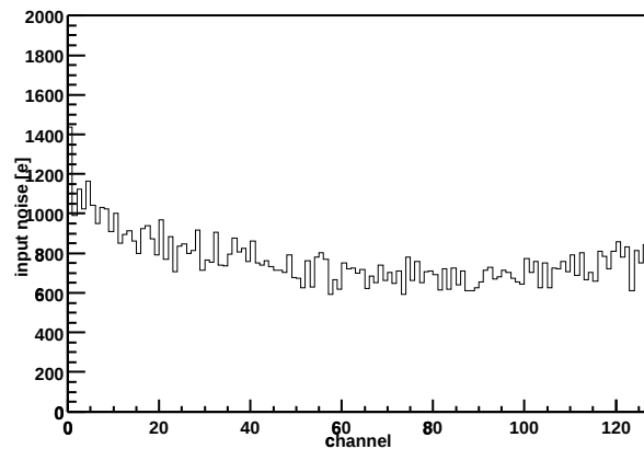
Chip Z36459A-W03-X02-Y10 Input noise vs. channel
