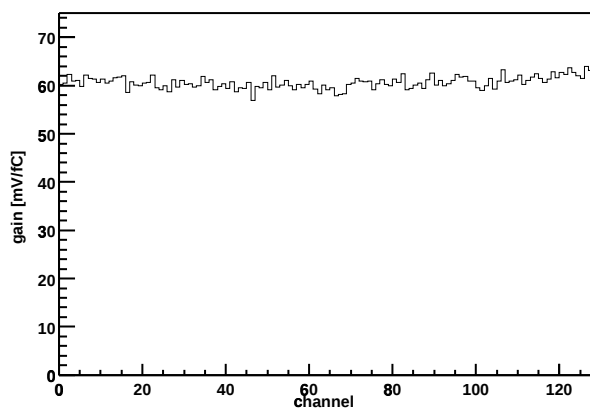
Chip Z36459A-W03-X02-Y10 Gain vs. channel
