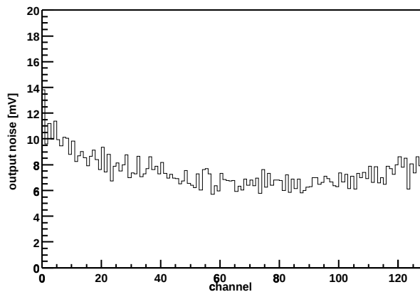
Chip Z36459A-W03-X02-Y10 Output noise vs. channel
