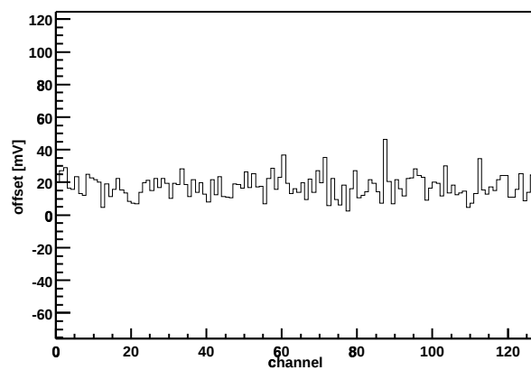
Chip Z36459A-W03-X02-Y11 Offset vs. channel
