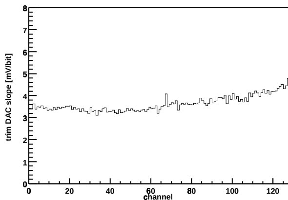
Chip Z36459A-W03-X02-Y11 Trim DAC slope vs. channel
