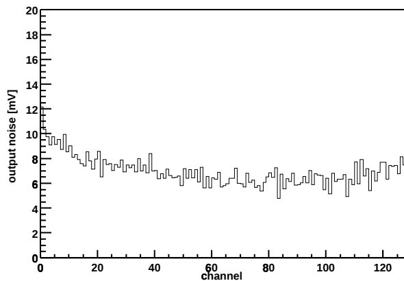
Chip Z36459A-W03-X02-Y11 Output noise vs. channel
