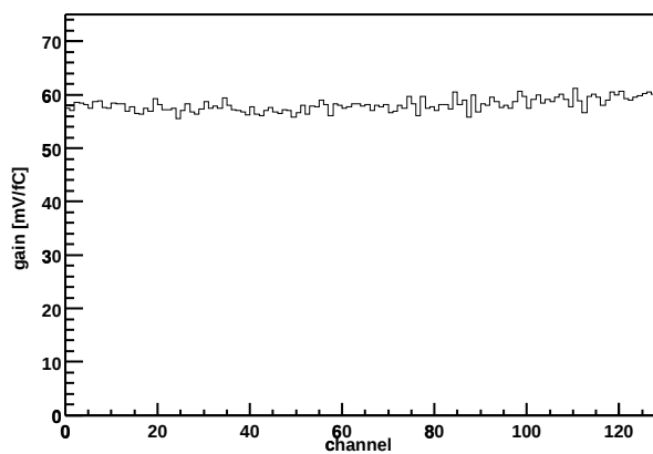
Chip Z36459A-W03-X02-Y11 Gain vs. channel
