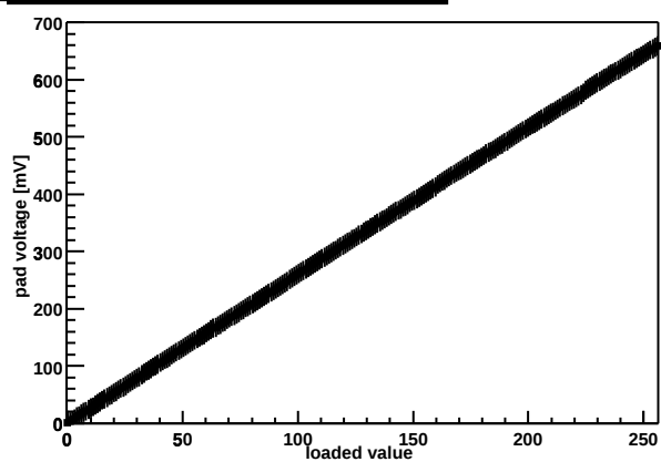
Chip Z36459A-W03-X02-Y11 threshold DAC
