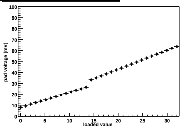
Chip Z36459A-W03-X02-Y11 shaper DAC
