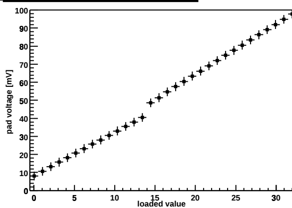
Chip Z36459A-W03-X02-Y11 preamp DAC
