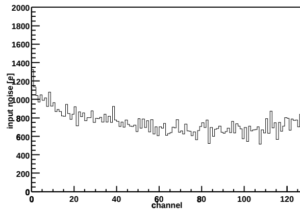
Chip Z36459A-W03-X02-Y11 Input noise vs. channel
