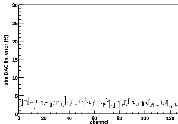
Chip Z36459A-W03-X02-Y11 trim DAC lin. error
