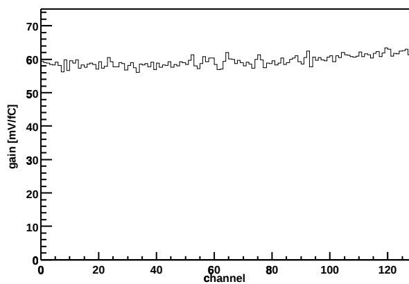
Chip Z36459A-W03-X02-Y12 Gain vs. channel
