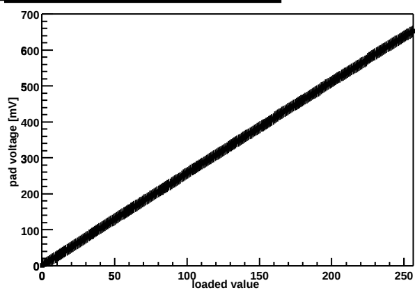
Chip Z36459A-W03-X02-Y12 threshold DAC
