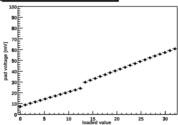
Chip Z36459A-W03-X02-Y12 shaper DAC
