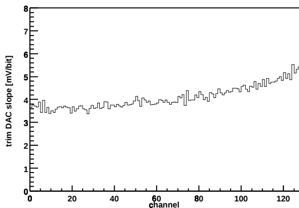
Chip Z36459A-W03-X02-Y12 Trim DAC slope vs. channel
