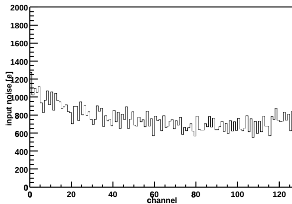
Chip Z36459A-W03-X02-Y12 Input noise vs. channel
