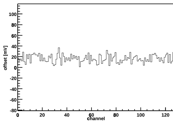
Chip Z36459A-W03-X02-Y12 Offset vs. channel
