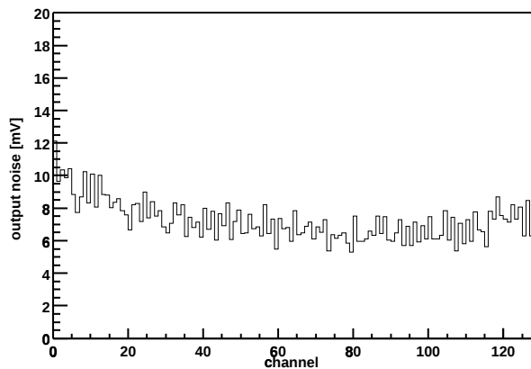
Chip Z36459A-W03-X02-Y12 Output noise vs. channel
