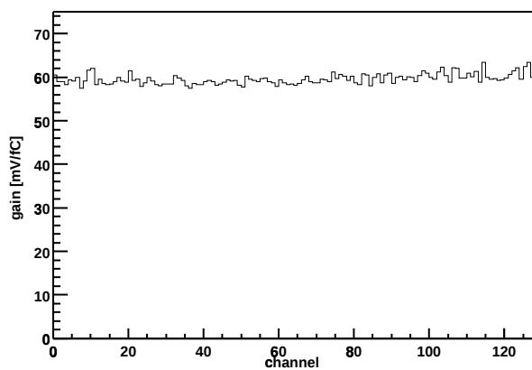
Chip Z36459A-W03-X02-Y13 Gain vs. channel
