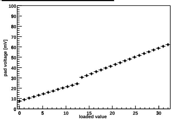
Chip Z36459A-W03-X02-Y13 shaper DAC
