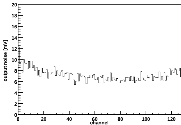
Chip Z36459A-W03-X02-Y13 Output noise vs. channel
