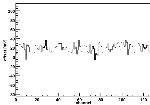
Chip Z36459A-W03-X02-Y13 Offset vs. channel
