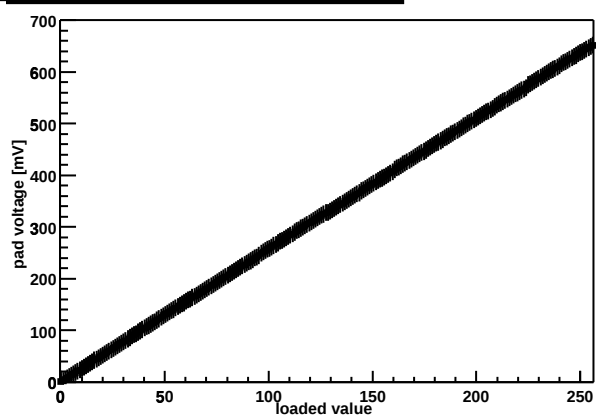
Chip Z36459A-W03-X02-Y13 threshold DAC
