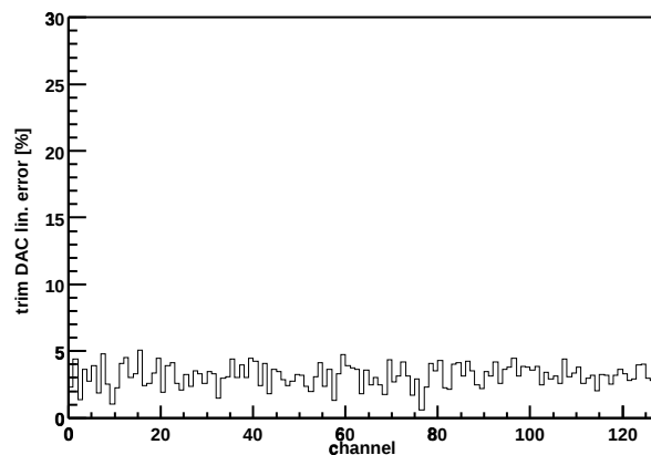
Chip Z36459A-W03-X02-Y13 trim DAC lin. error
