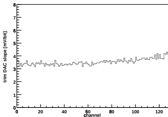
Chip Z36459A-W03-X02-Y13 Trim DAC slope vs. channel
