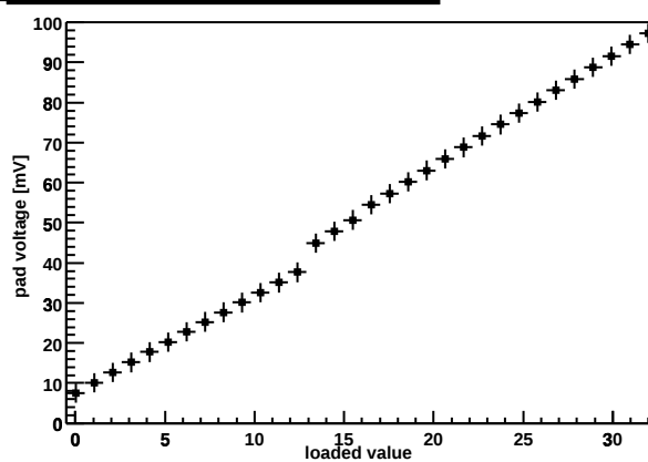
Chip Z36459A-W03-X02-Y13 preamp DAC
