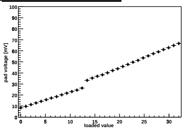
Chip Z36459A-W03-X03-Y04 shaper DAC
