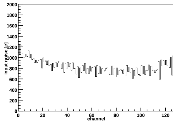
Chip Z36459A-W03-X03-Y04 Input noise vs. channel
