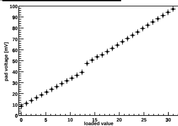
Chip Z36459A-W03-X03-Y04 preamp DAC
