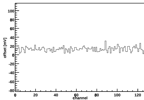
Chip Z36459A-W03-X03-Y04 Offset vs. channel
