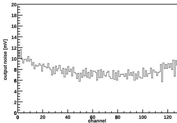
Chip Z36459A-W03-X03-Y04 Output noise vs. channel
