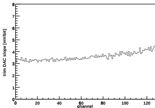
Chip Z36459A-W03-X03-Y04 Trim DAC slope vs. channel
