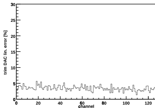
Chip Z36459A-W03-X03-Y04 trim DAC lin. error
