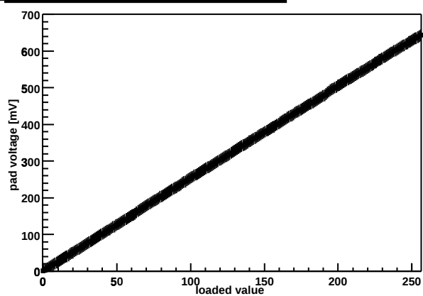
Chip Z36459A-W03-X03-Y04 threshold DAC
