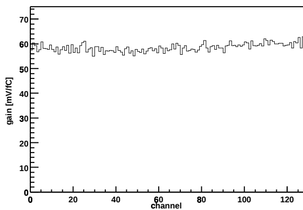
Chip Z36459A-W03-X03-Y04 Gain vs. channel
