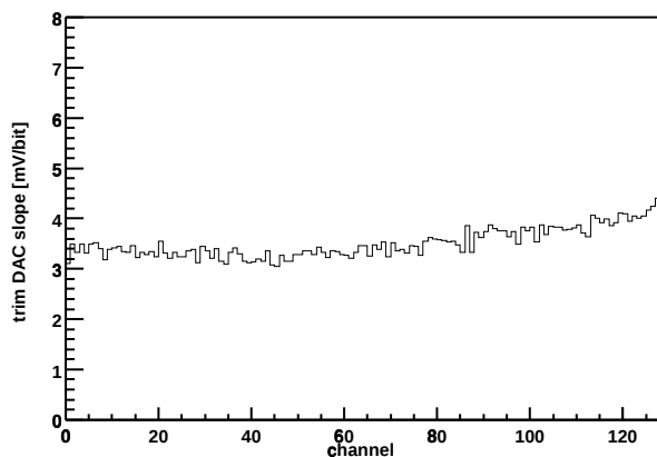
Chip Z36459A-W03-X03-Y11 Trim DAC slope vs. channel
