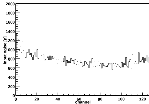
Chip Z36459A-W03-X03-Y11 Input noise vs. channel
