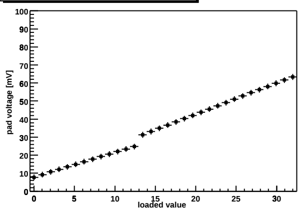
Chip Z36459A-W03-X03-Y11 shaper DAC
