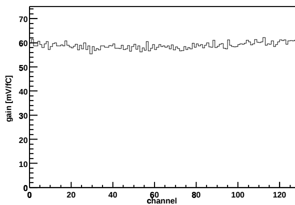
Chip Z36459A-W03-X03-Y11 Gain vs. channel
