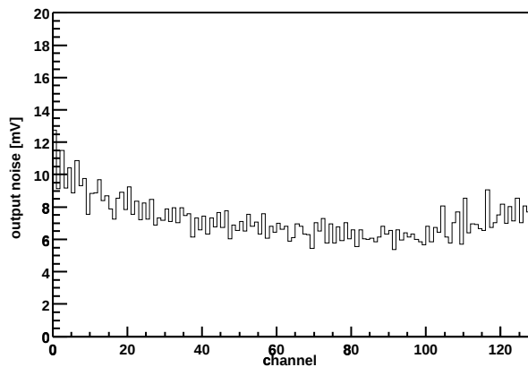
Chip Z36459A-W03-X03-Y11 Output noise vs. channel
