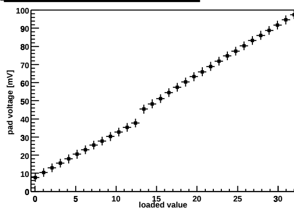
Chip Z36459A-W03-X03-Y11 preamp DAC
