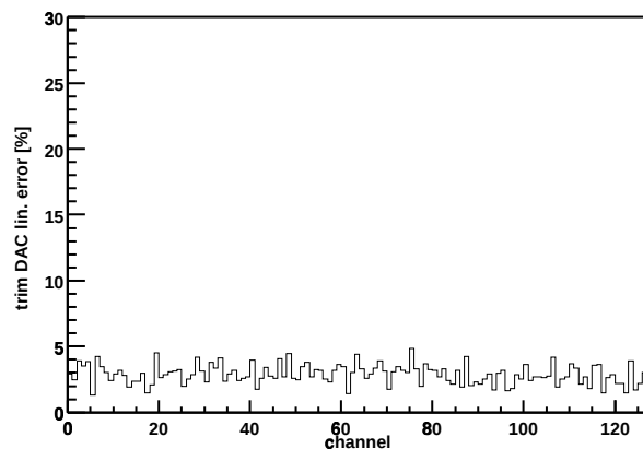
Chip Z36459A-W03-X03-Y11 trim DAC lin. error
