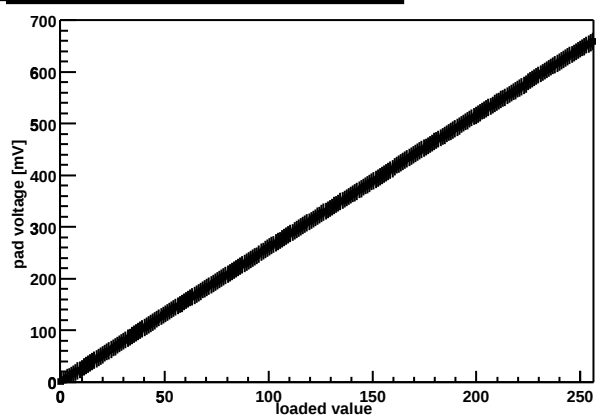
Chip Z36459A-W03-X03-Y11 threshold DAC
