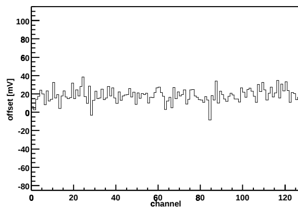
Chip Z36459A-W03-X03-Y14 Offset vs. channel
