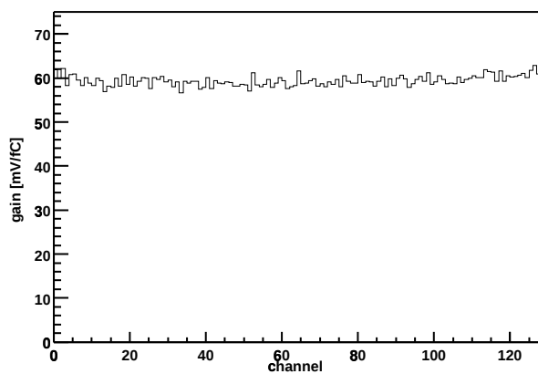
Chip Z36459A-W03-X03-Y14 Gain vs. channel
