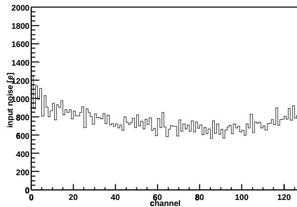
Chip Z36459A-W03-X03-Y14 Input noise vs. channel
