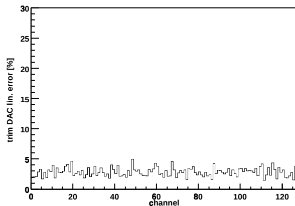
Chip Z36459A-W03-X03-Y14 trim DAC lin. error
