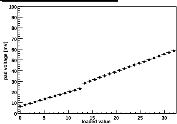
Chip Z36459A-W03-X03-Y14 shaper DAC
