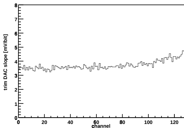
Chip Z36459A-W03-X03-Y14 Trim DAC slope vs. channel
