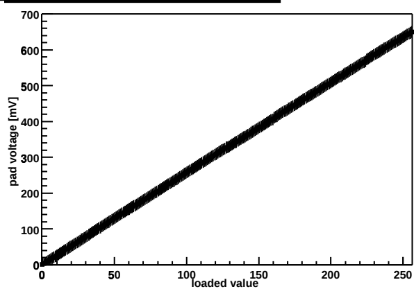
Chip Z36459A-W03-X03-Y14 threshold DAC
