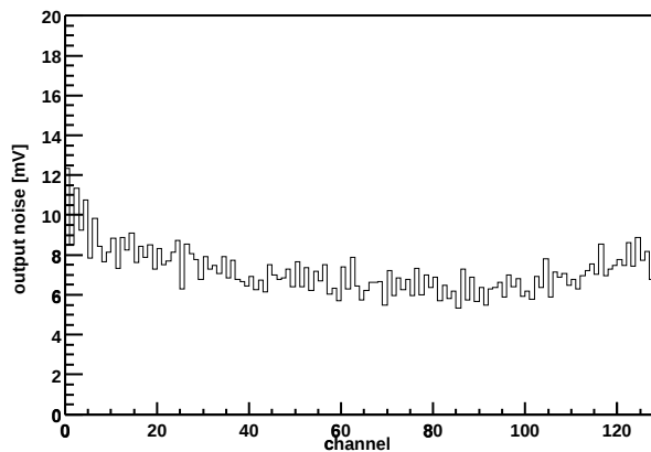
Chip Z36459A-W03-X03-Y14 Output noise vs. channel
