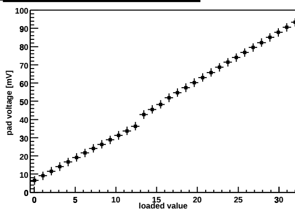
Chip Z36459A-W03-X03-Y14 preamp DAC
