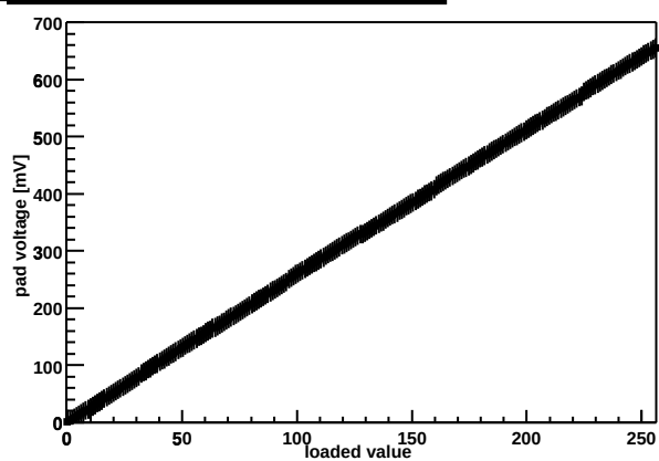
Chip Z36459A-W03-X03-Y15 threshold DAC
