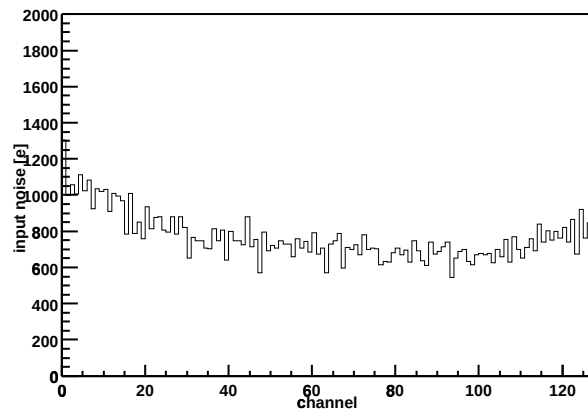
Chip Z36459A-W03-X03-Y15 Input noise vs. channel
