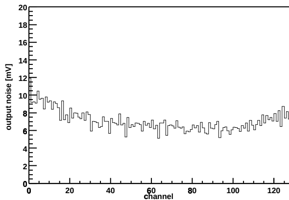
Chip Z36459A-W03-X03-Y15 Output noise vs. channel
