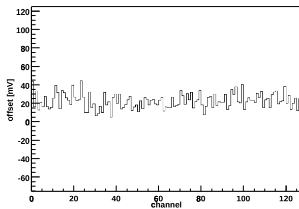
Chip Z36459A-W03-X03-Y15 Offset vs. channel
