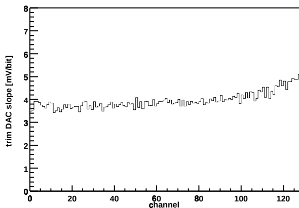
Chip Z36459A-W03-X03-Y15 Trim DAC slope vs. channel
