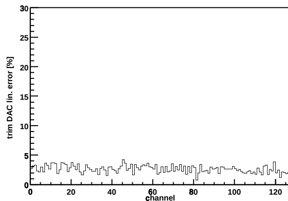
Chip Z36459A-W03-X03-Y15 trim DAC lin. error
