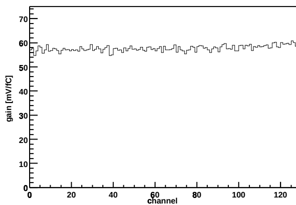
Chip Z36459A-W03-X03-Y15 Gain vs. channel
