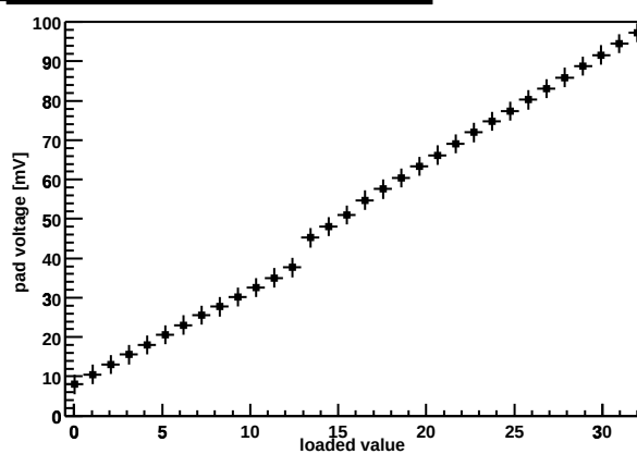
Chip Z36459A-W03-X03-Y16 preamp DAC
