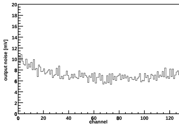
Chip Z36459A-W03-X03-Y16 Output noise vs. channel
