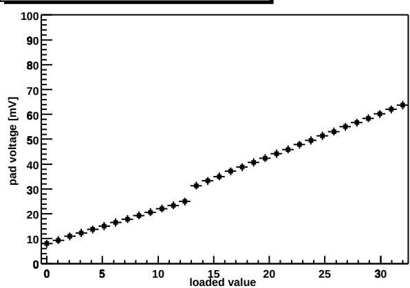
Chip Z36459A-W03-X03-Y16 shaper DAC
