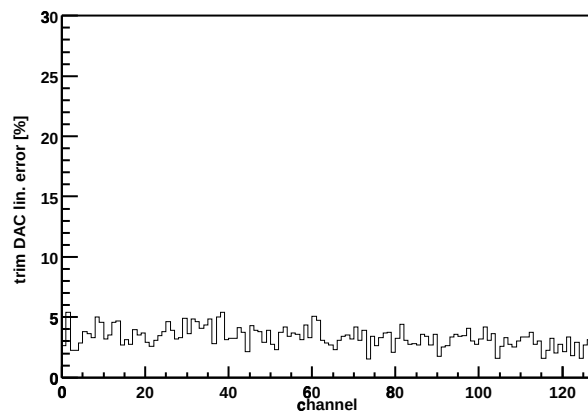
Chip Z36459A-W03-X03-Y16 trim DAC lin. error
