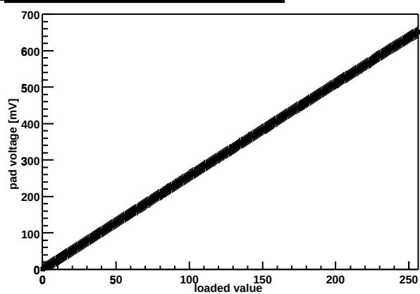
Chip Z36459A-W03-X03-Y16 threshold DAC
