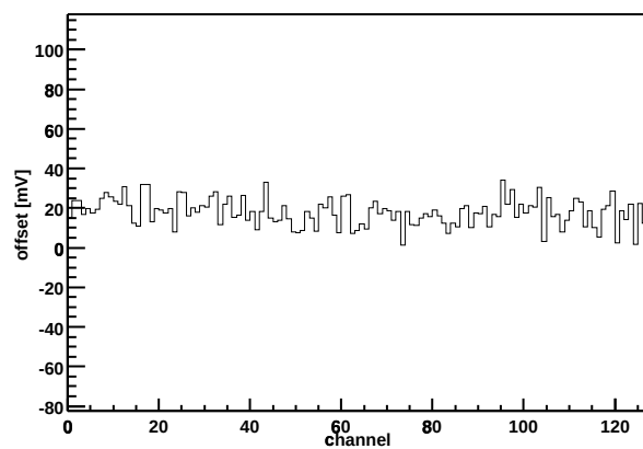
Chip Z36459A-W03-X03-Y16 Offset vs. channel
