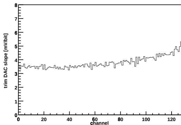
Chip Z36459A-W03-X03-Y16 Trim DAC slope vs. channel
