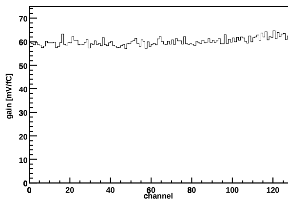
Chip Z36459A-W03-X03-Y16 Gain vs. channel
