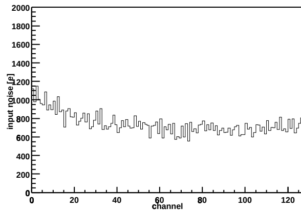
Chip Z36459A-W03-X03-Y16 Input noise vs. channel
