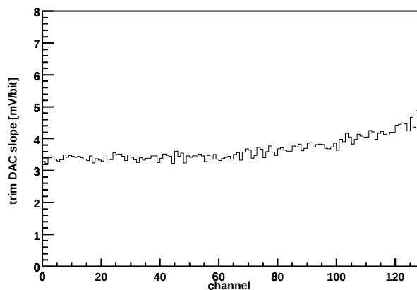
Chip Z36459A-W03-X04-Y07 Trim DAC slope vs. channel
