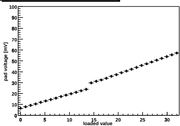
Chip Z36459A-W03-X04-Y07 shaper DAC
