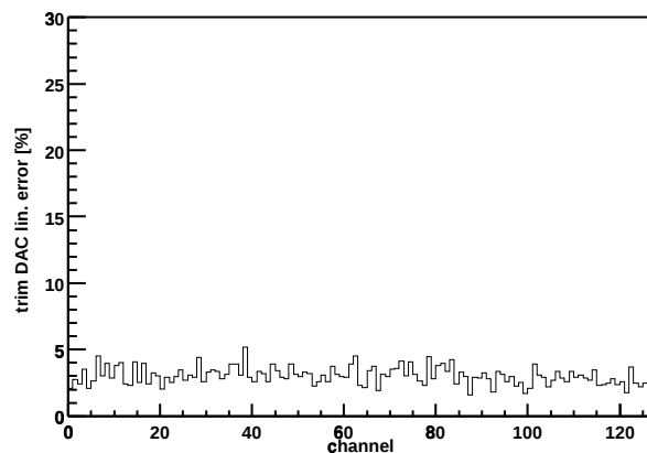
Chip Z36459A-W03-X04-Y07 trim DAC lin. error
