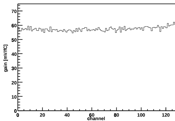
Chip Z36459A-W03-X04-Y07 Gain vs. channel
