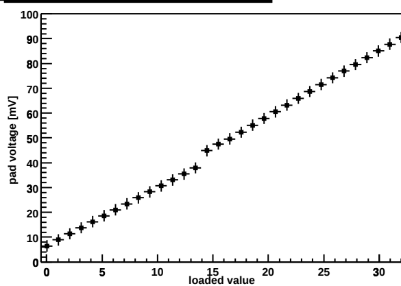
Chip Z36459A-W03-X04-Y07 preamp DAC
