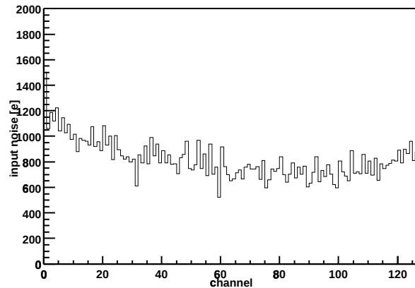
Chip Z36459A-W03-X04-Y07 Input noise vs. channel
