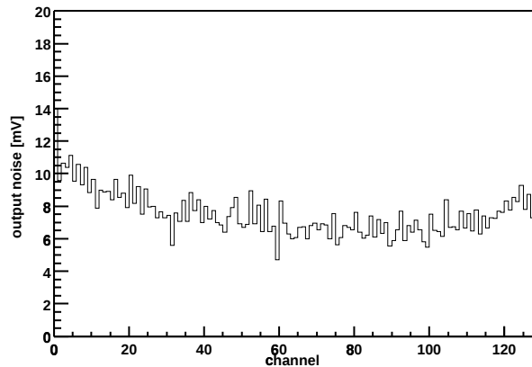
Chip Z36459A-W03-X04-Y07 Output noise vs. channel
