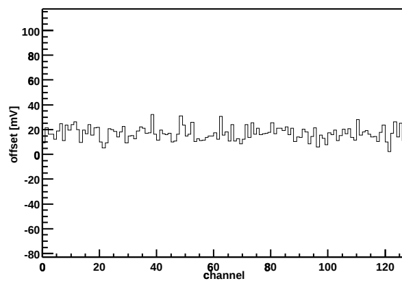
Chip Z36459A-W03-X04-Y07 Offset vs. channel
