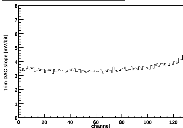
Chip Z36459A-W03-X04-Y09 Trim DAC slope vs. channel
