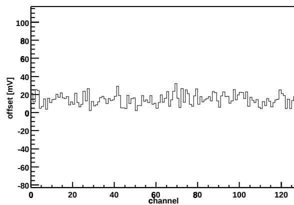
Chip Z36459A-W03-X04-Y09 Offset vs. channel
