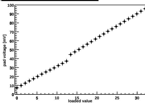
Chip Z36459A-W03-X04-Y09 preamp DAC
