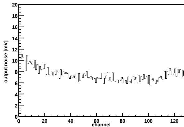
Chip Z36459A-W03-X04-Y09 Output noise vs. channel
