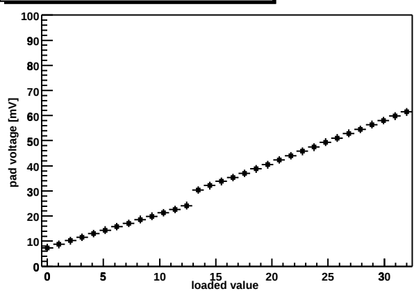
Chip Z36459A-W03-X04-Y09 shaper DAC
