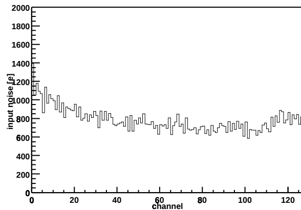
Chip Z36459A-W03-X04-Y09 Input noise vs. channel
