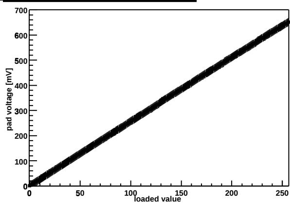
Chip Z36459A-W03-X04-Y09 threshold DAC
