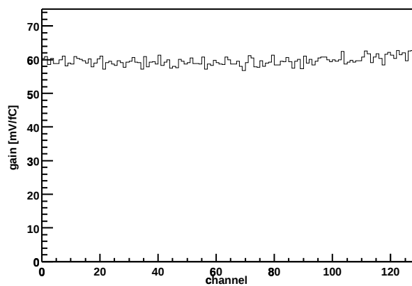
Chip Z36459A-W03-X04-Y09 Gain vs. channel
