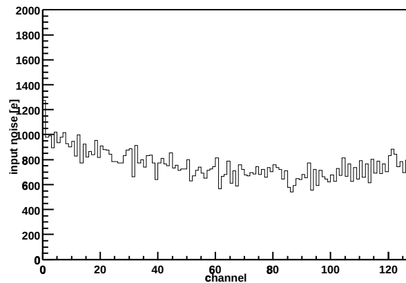
Chip Z36459A-W03-X04-Y14 Input noise vs. channel
