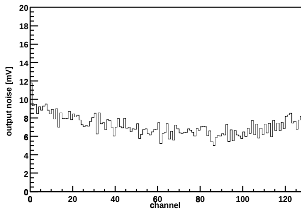
Chip Z36459A-W03-X04-Y14 Output noise vs. channel
