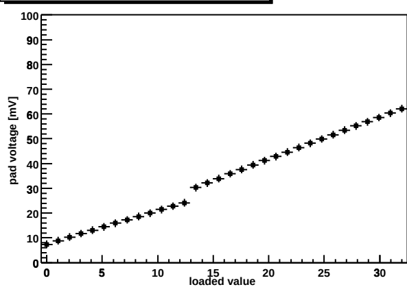
Chip Z36459A-W03-X04-Y14 shaper DAC
