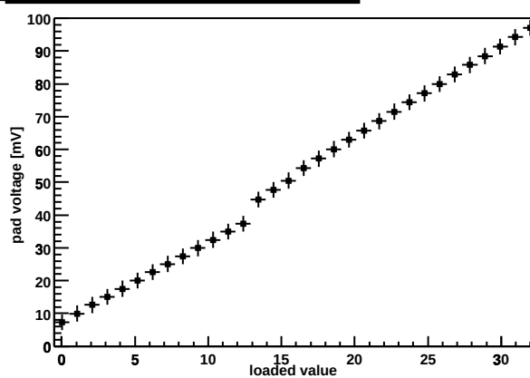
Chip Z36459A-W03-X04-Y14 preamp DAC
