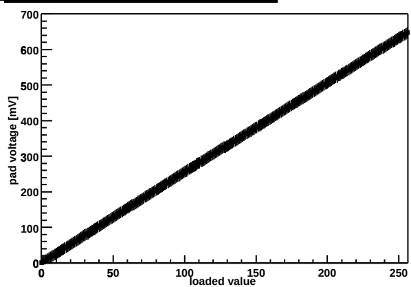
Chip Z36459A-W03-X04-Y14 threshold DAC
