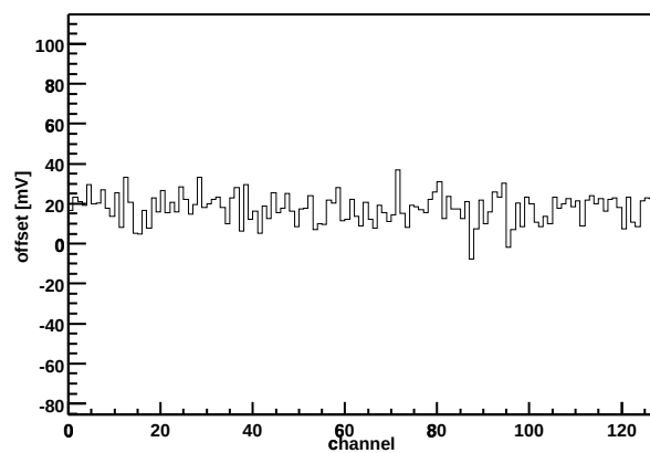
Chip Z36459A-W03-X04-Y14 Offset vs. channel
