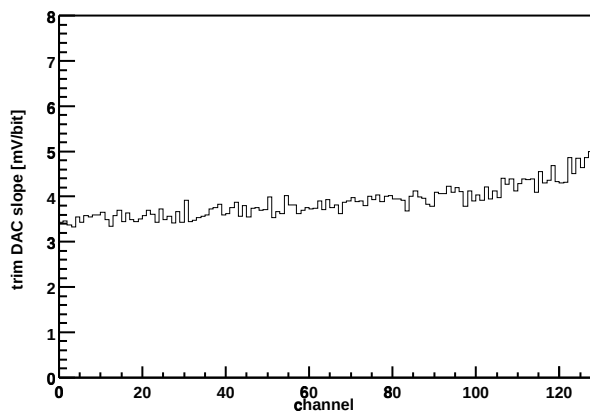
Chip Z36459A-W03-X04-Y14 Trim DAC slope vs. channel
