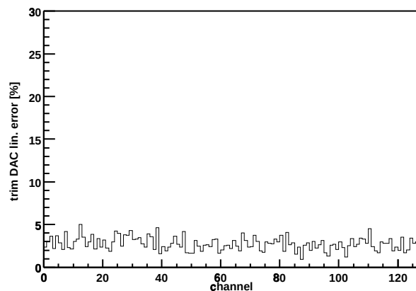
Chip Z36459A-W03-X04-Y14 trim DAC lin. error
