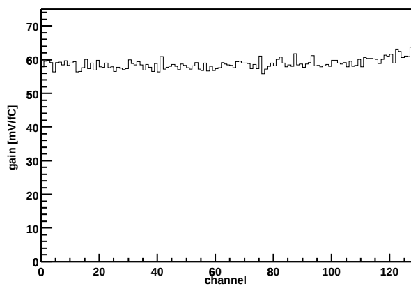
Chip Z36459A-W03-X04-Y14 Gain vs. channel
