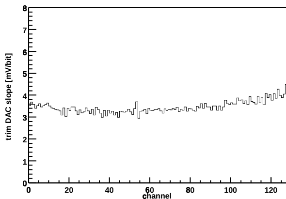
Chip Z36459A-W03-X05-Y03 Trim DAC slope vs. channel
