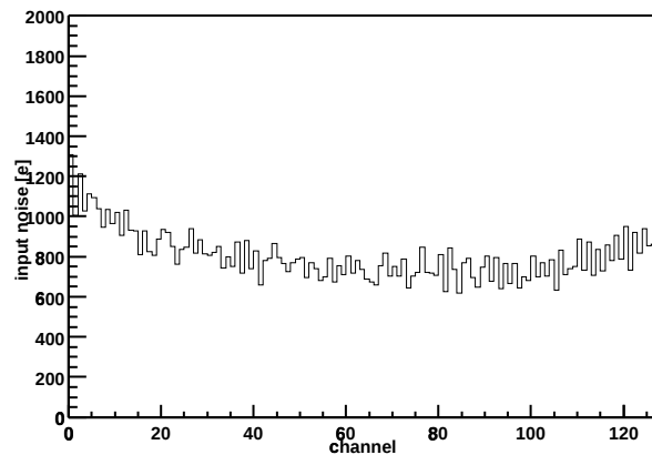
Chip Z36459A-W03-X05-Y03 Input noise vs. channel
