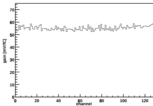
Chip Z36459A-W03-X05-Y03 Gain vs. channel
