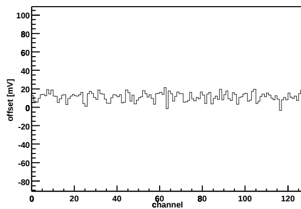
Chip Z36459A-W03-X05-Y03 Offset vs. channel
