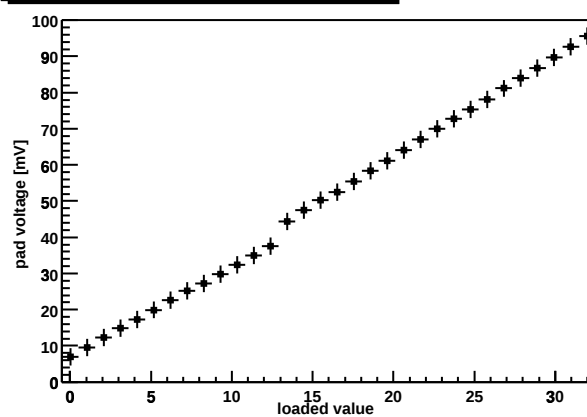
Chip Z36459A-W03-X05-Y03 preamp DAC
