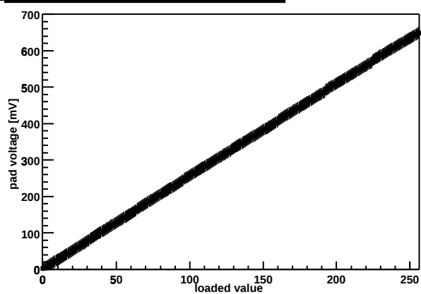
Chip Z36459A-W03-X05-Y03 threshold DAC
