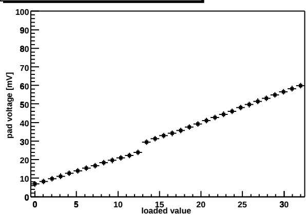
Chip Z36459A-W03-X05-Y03 shaper DAC
