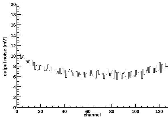
Chip Z36459A-W03-X05-Y03 Output noise vs. channel
