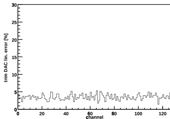
Chip Z36459A-W03-X05-Y03 trim DAC lin. error
