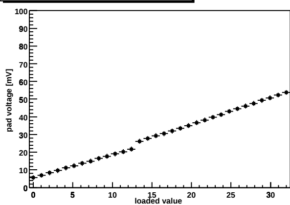
Chip Z36459A-W03-X05-Y06 shaper DAC
