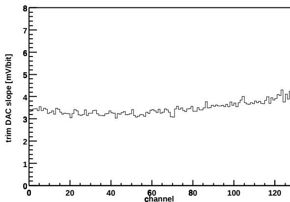
Chip Z36459A-W03-X05-Y06 Trim DAC slope vs. channel
