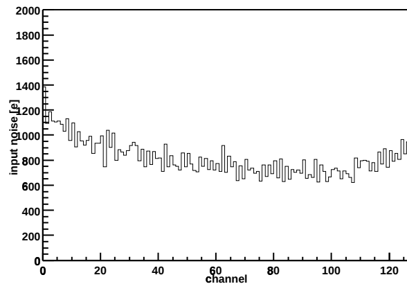
Chip Z36459A-W03-X05-Y06 Input noise vs. channel
