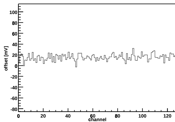
Chip Z36459A-W03-X05-Y06 Offset vs. channel
