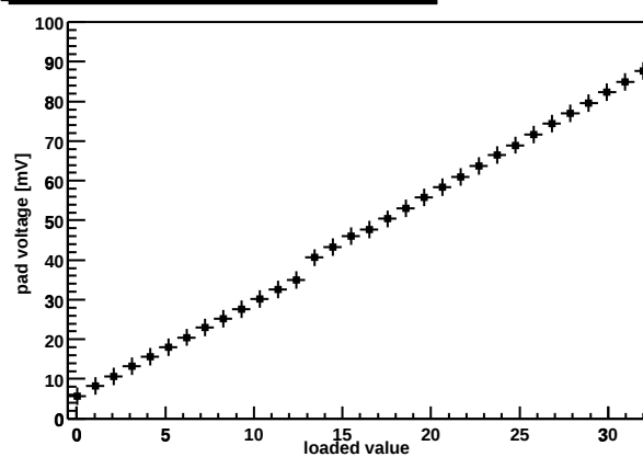
Chip Z36459A-W03-X05-Y06 preamp DAC
