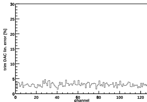
Chip Z36459A-W03-X05-Y06 trim DAC lin. error
