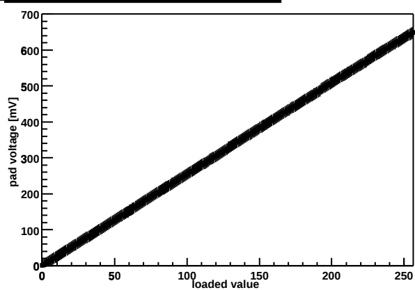
Chip Z36459A-W03-X05-Y06 threshold DAC
