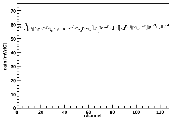
Chip Z36459A-W03-X05-Y06 Gain vs. channel
