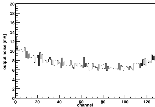
Chip Z36459A-W03-X05-Y06 Output noise vs. channel
