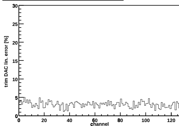
Chip Z36459A-W03-X05-Y08 trim DAC lin. error
