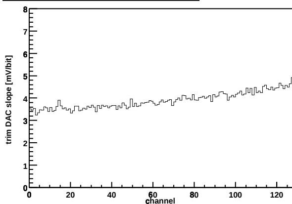
Chip Z36459A-W03-X05-Y08 Trim DAC slope vs. channel
