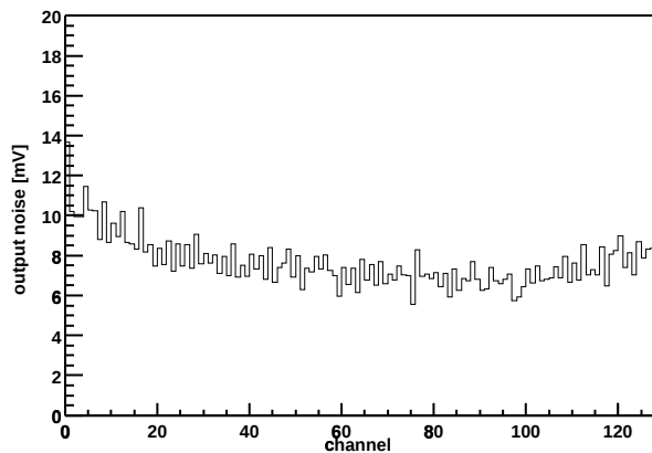
Chip Z36459A-W03-X05-Y08 Output noise vs. channel
