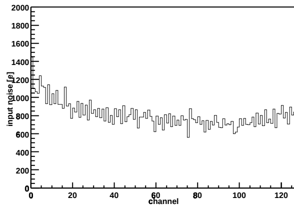
Chip Z36459A-W03-X05-Y08 Input noise vs. channel
