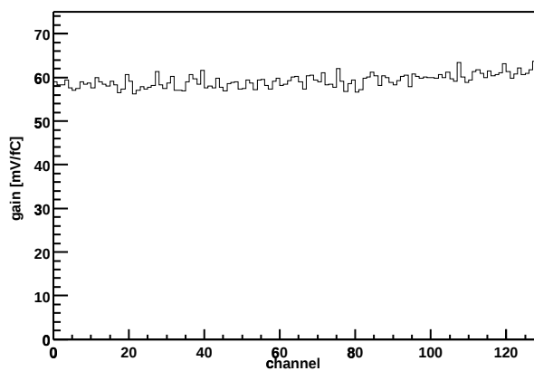
Chip Z36459A-W03-X05-Y08 Gain vs. channel
