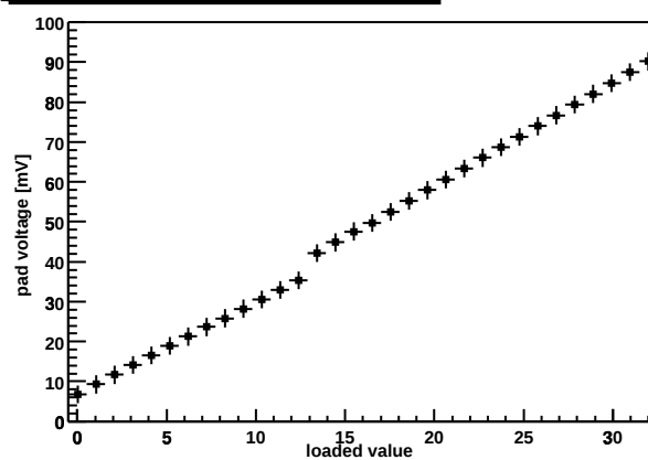
Chip Z36459A-W03-X05-Y08 preamp DAC
