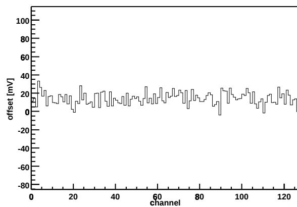
Chip Z36459A-W03-X05-Y08 Offset vs. channel
