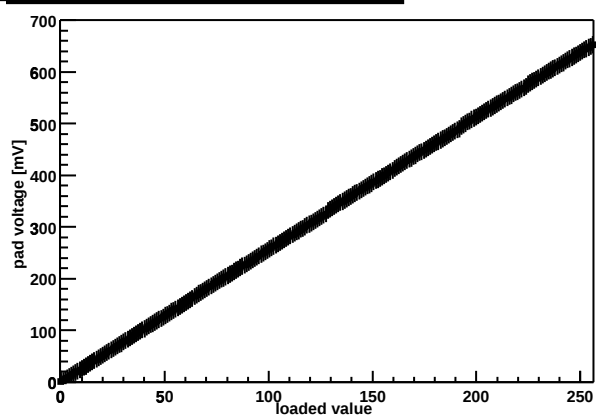
Chip Z36459A-W03-X05-Y08 threshold DAC
