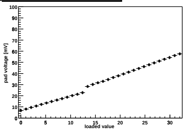
Chip Z36459A-W03-X05-Y08 shaper DAC
