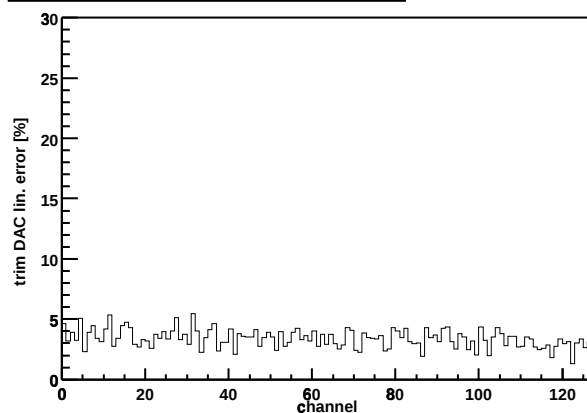
Chip Z36459A-W03-X05-Y10 trim DAC lin. error
