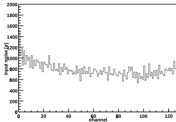
Chip Z36459A-W03-X05-Y10 Input noise vs. channel
