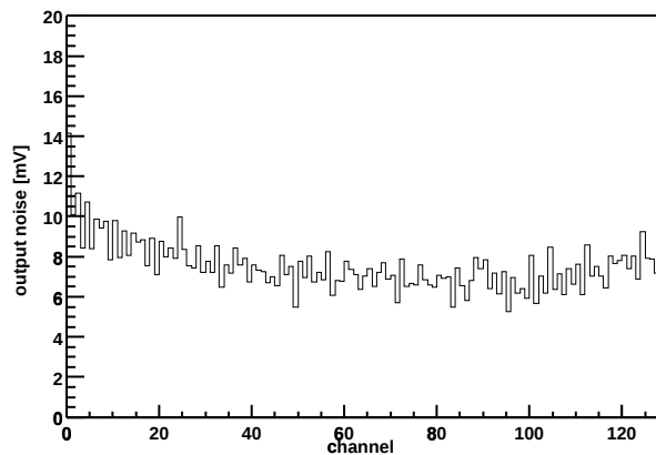
Chip Z36459A-W03-X05-Y10 Output noise vs. channel
