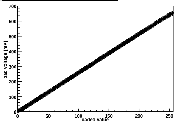
Chip Z36459A-W03-X05-Y10 threshold DAC
