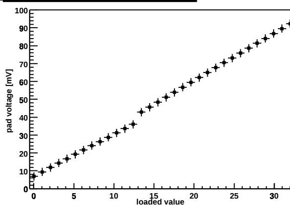
Chip Z36459A-W03-X05-Y10 preamp DAC
