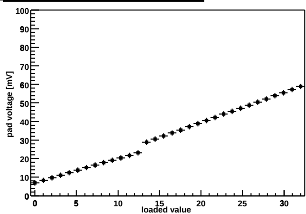
Chip Z36459A-W03-X05-Y10 shaper DAC
