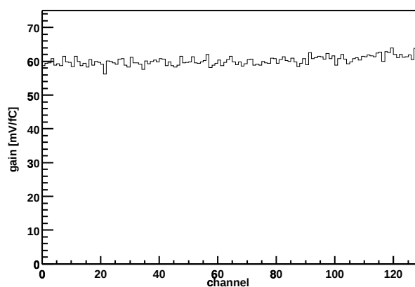
Chip Z36459A-W03-X05-Y10 Gain vs. channel
