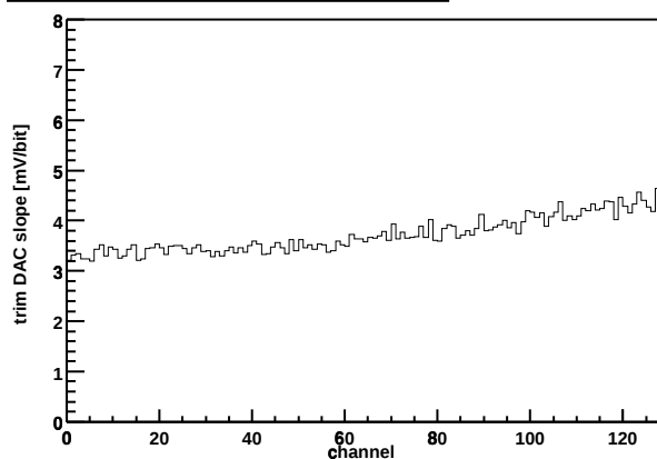
Chip Z36459A-W03-X05-Y10 Trim DAC slope vs. channel
