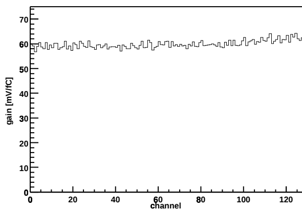
Chip Z36459A-W03-X05-Y13 Gain vs. channel
