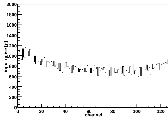
Chip Z36459A-W03-X05-Y13 Input noise vs. channel
