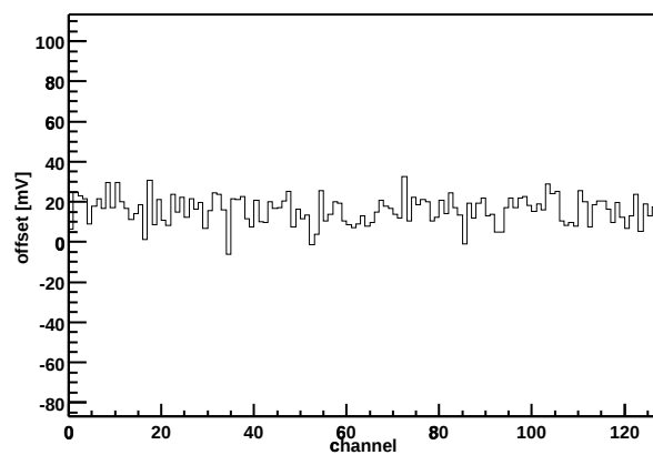
Chip Z36459A-W03-X05-Y13 Offset vs. channel
