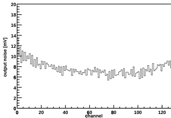
Chip Z36459A-W03-X05-Y13 Output noise vs. channel
