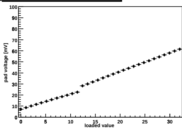
Chip Z36459A-W03-X05-Y13 shaper DAC
