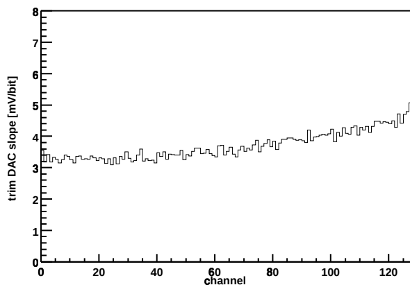
Chip Z36459A-W03-X05-Y13 Trim DAC slope vs. channel
