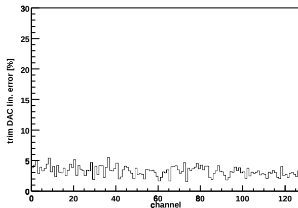
Chip Z36459A-W03-X05-Y13 trim DAC lin. error
