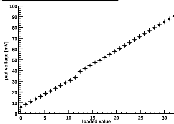
Chip Z36459A-W03-X06-Y06 preamp DAC
