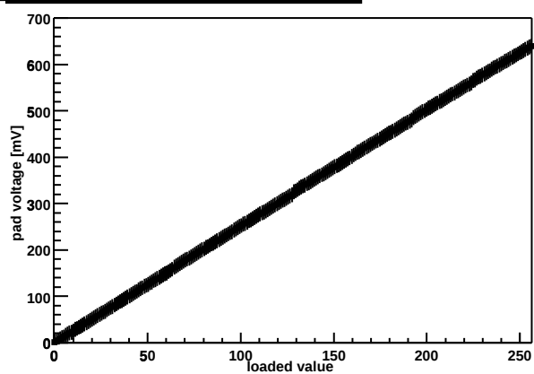
Chip Z36459A-W03-X06-Y06 threshold DAC
