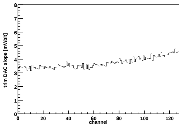
Chip Z36459A-W03-X06-Y06 Trim DAC slope vs. channel
