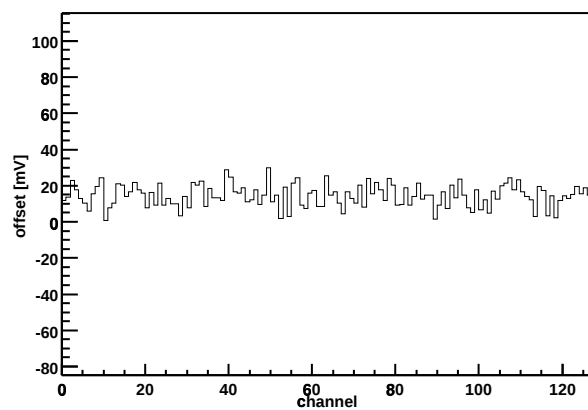
Chip Z36459A-W03-X06-Y06 Offset vs. channel
