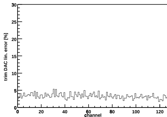
Chip Z36459A-W03-X06-Y06 trim DAC lin. error
