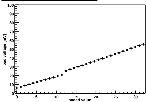
Chip Z36459A-W03-X06-Y06 shaper DAC
