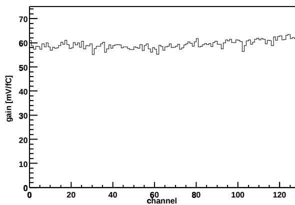
Chip Z36459A-W03-X06-Y06 Gain vs. channel
