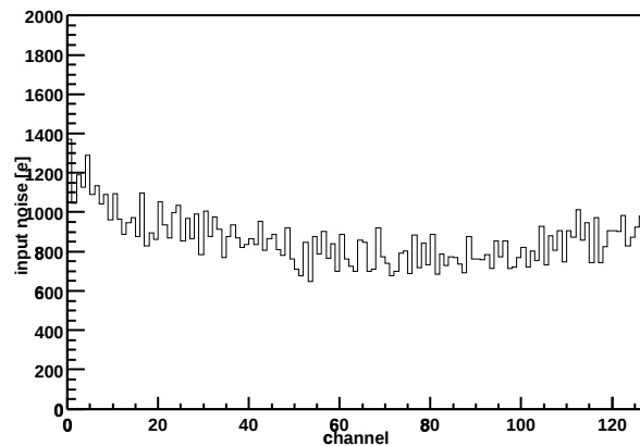
Chip Z36459A-W03-X06-Y06 Input noise vs. channel
