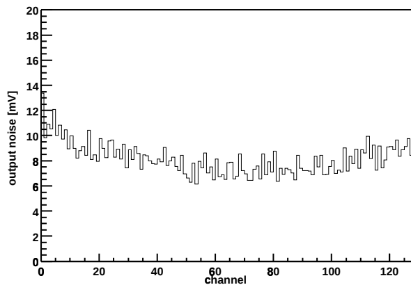
Chip Z36459A-W03-X06-Y06 Output noise vs. channel
