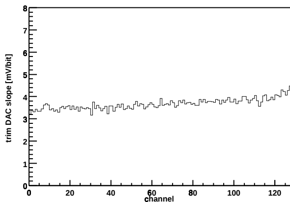
Chip Z36459A-W03-X06-Y09 Trim DAC slope vs. channel
