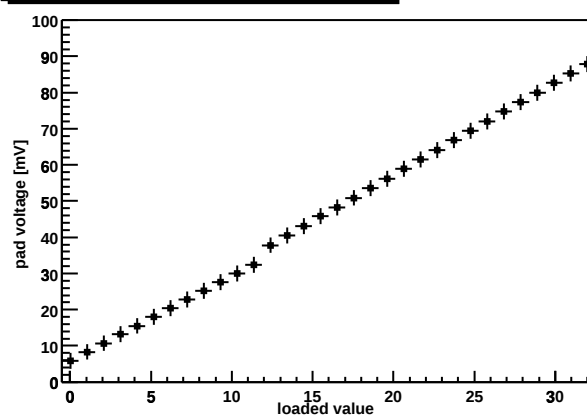
Chip Z36459A-W03-X06-Y09 preamp DAC
