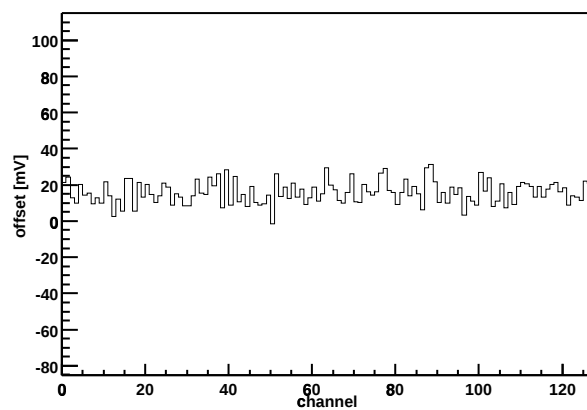
Chip Z36459A-W03-X06-Y09 Offset vs. channel
