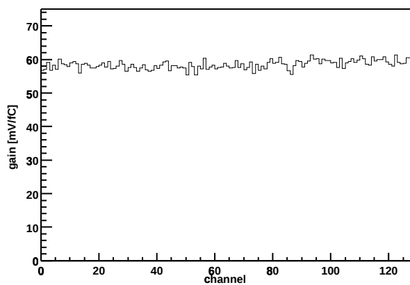
Chip Z36459A-W03-X06-Y09 Gain vs. channel
