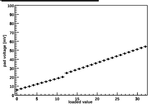
Chip Z36459A-W03-X06-Y09 shaper DAC
