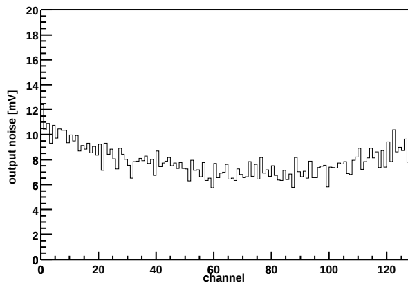
Chip Z36459A-W03-X06-Y09 Output noise vs. channel
