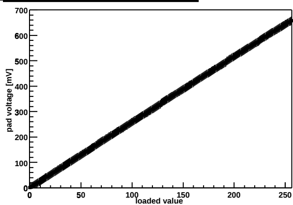
Chip Z36459A-W03-X06-Y09 threshold DAC
