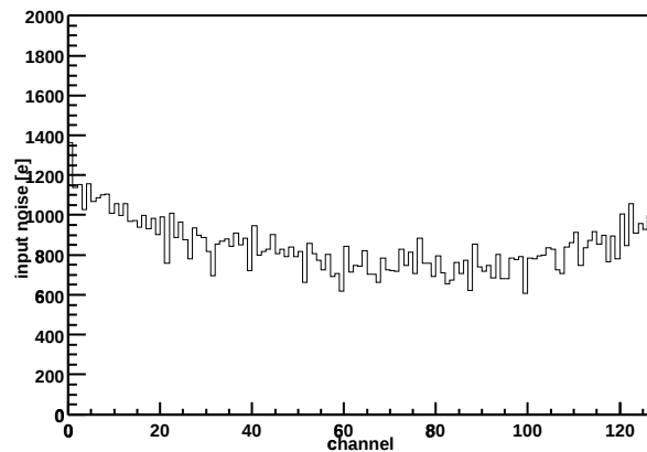
Chip Z36459A-W03-X06-Y09 Input noise vs. channel
