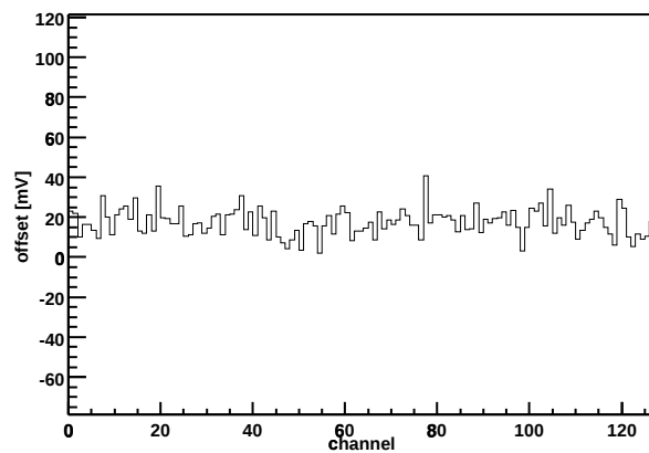
Chip Z36459A-W03-X06-Y19 Offset vs. channel
