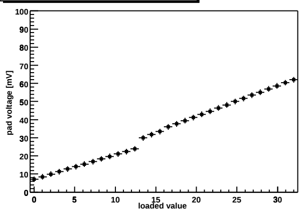
Chip Z36459A-W03-X06-Y19 shaper DAC
