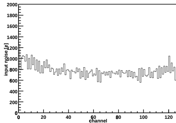
Chip Z36459A-W03-X06-Y19 Input noise vs. channel
