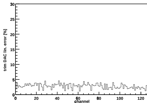
Chip Z36459A-W03-X06-Y19 trim DAC lin. error
