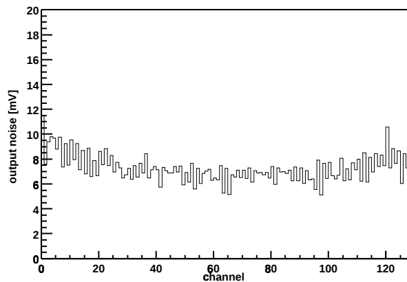
Chip Z36459A-W03-X06-Y19 Output noise vs. channel
