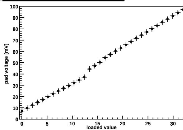
Chip Z36459A-W03-X06-Y19 preamp DAC
