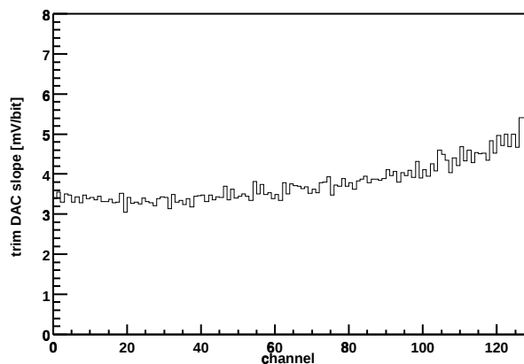
Chip Z36459A-W03-X06-Y19 Trim DAC slope vs. channel
