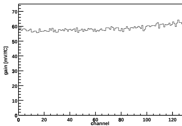
Chip Z36459A-W03-X06-Y19 Gain vs. channel
