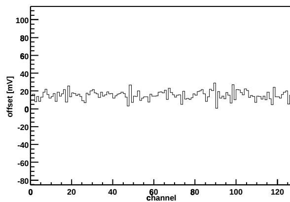
Chip Z36459A-W03-X07-Y02 Offset vs. channel
