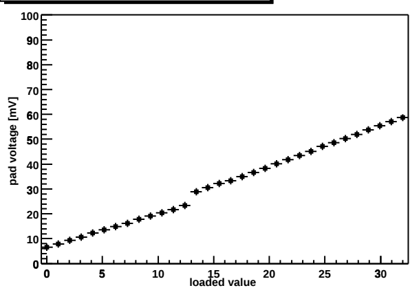
Chip Z36459A-W03-X07-Y02 shaper DAC
