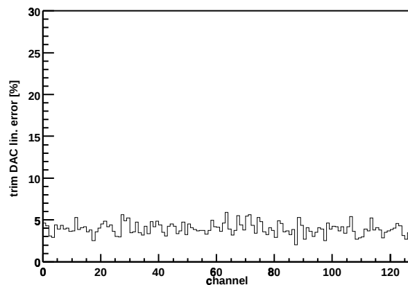
Chip Z36459A-W03-X07-Y02 trim DAC lin. error
