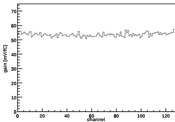
Chip Z36459A-W03-X07-Y02 Gain vs. channel
