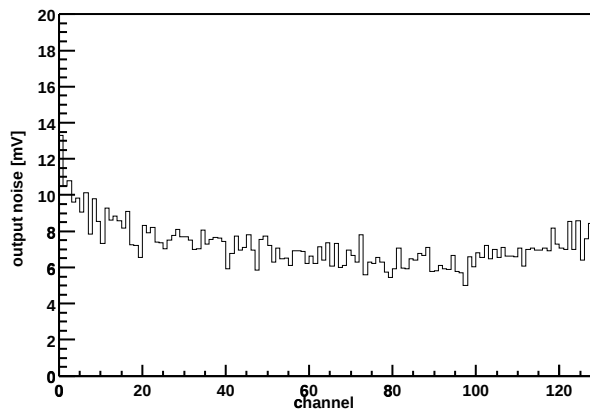
Chip Z36459A-W03-X07-Y02 Output noise vs. channel
