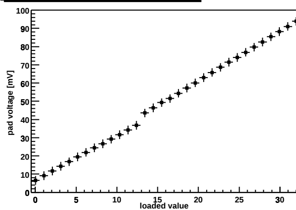
Chip Z36459A-W03-X07-Y02 preamp DAC
