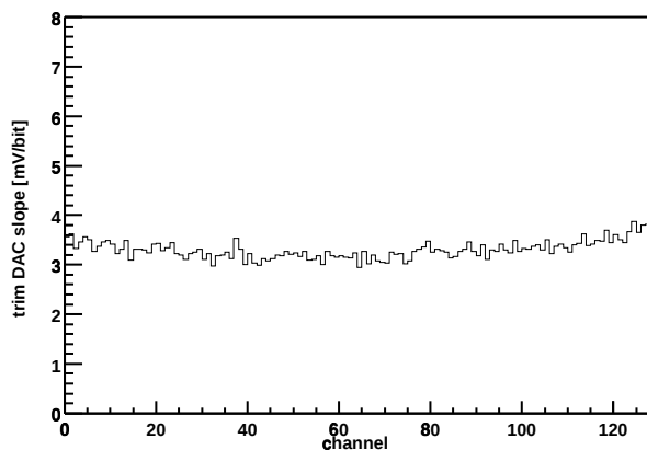
Chip Z36459A-W03-X07-Y02 Trim DAC slope vs. channel
