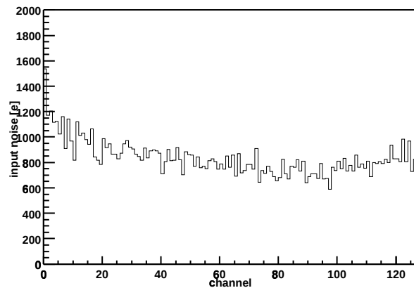
Chip Z36459A-W03-X07-Y02 Input noise vs. channel
