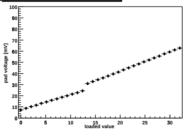
Chip Z36459A-W03-X07-Y05 shaper DAC
