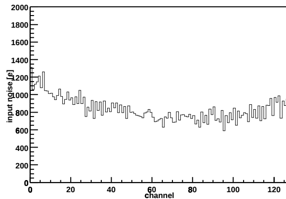
Chip Z36459A-W03-X07-Y05 Input noise vs. channel
