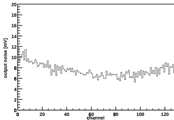
Chip Z36459A-W03-X07-Y05 Output noise vs. channel
