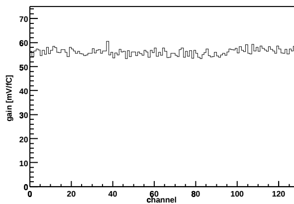
Chip Z36459A-W03-X07-Y05 Gain vs. channel
