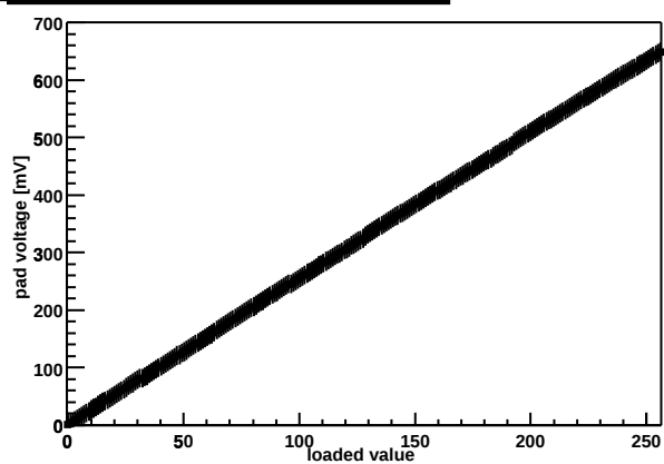
Chip Z36459A-W03-X07-Y05 threshold DAC
