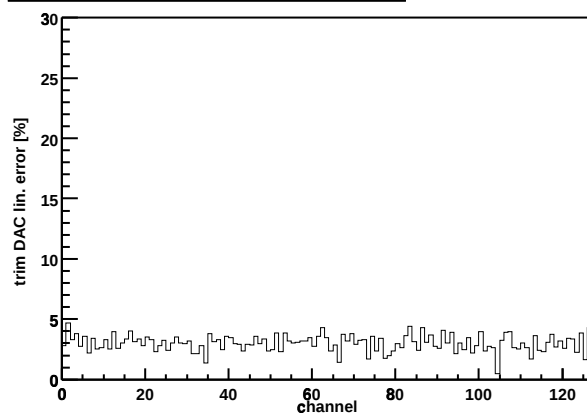
Chip Z36459A-W03-X07-Y05 trim DAC lin. error
