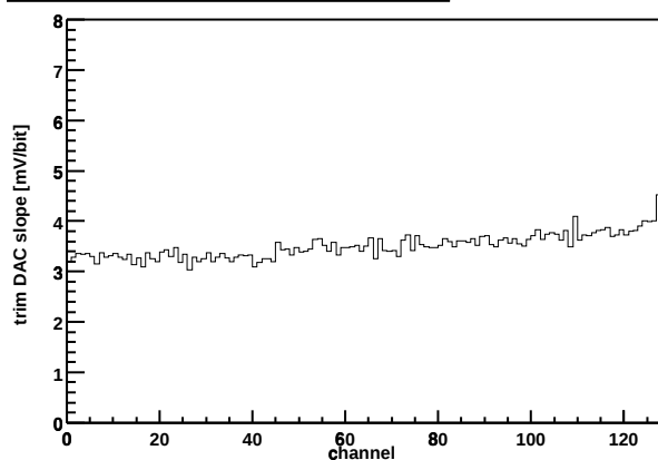
Chip Z36459A-W03-X07-Y05 Trim DAC slope vs. channel
