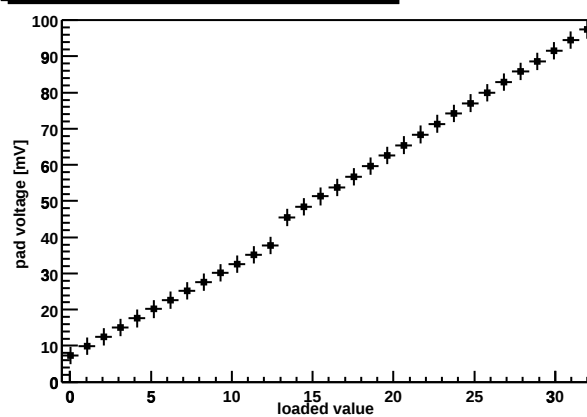
Chip Z36459A-W03-X07-Y05 preamp DAC
