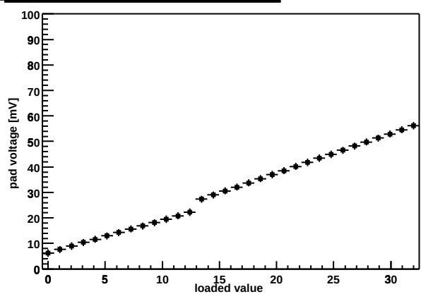
Chip Z36459A-W03-X07-Y09 shaper DAC
