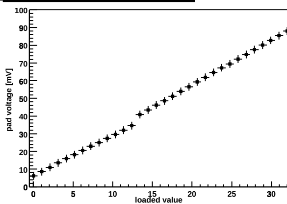
Chip Z36459A-W03-X07-Y09 preamp DAC
