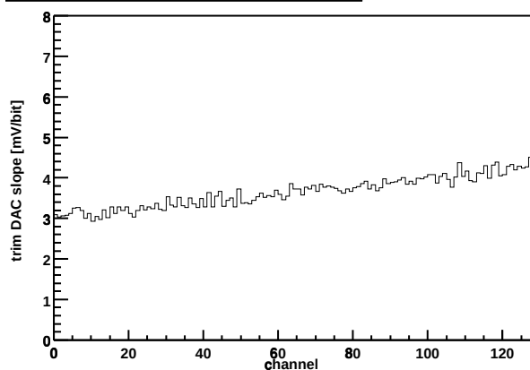
Chip Z36459A-W03-X07-Y09 Trim DAC slope vs. channel
