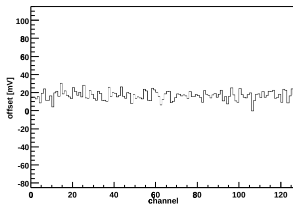
Chip Z36459A-W03-X07-Y09 Offset vs. channel
