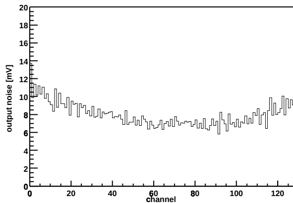
Chip Z36459A-W03-X07-Y09 Output noise vs. channel
