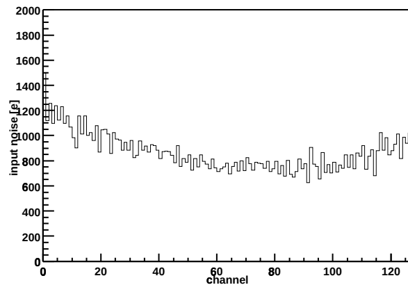
Chip Z36459A-W03-X07-Y09 Input noise vs. channel
