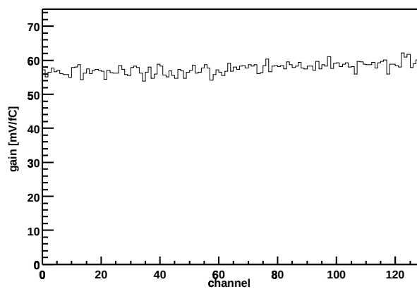
Chip Z36459A-W03-X07-Y09 Gain vs. channel
