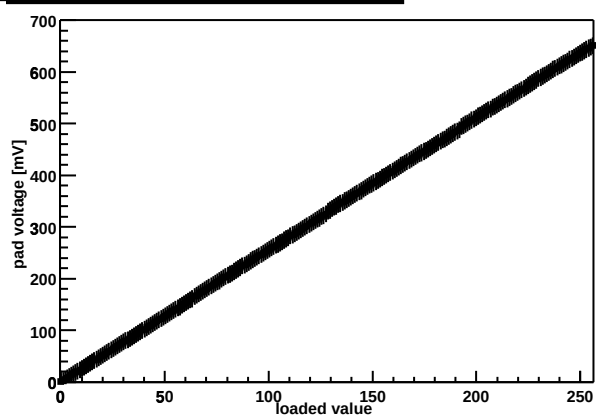
Chip Z36459A-W03-X07-Y09 threshold DAC
