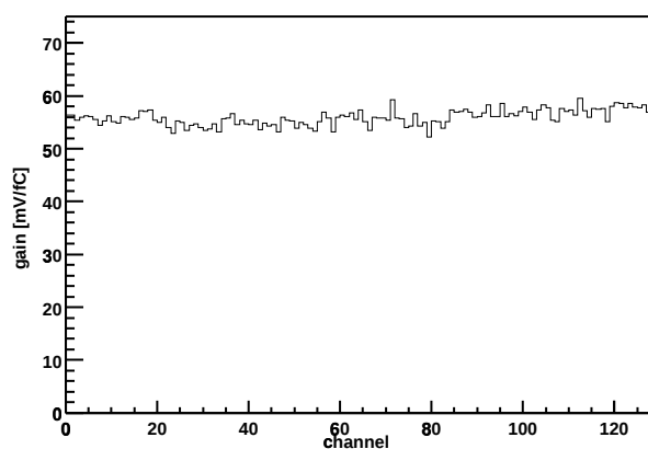
Chip Z36459A-W03-X09-Y04 Gain vs. channel
