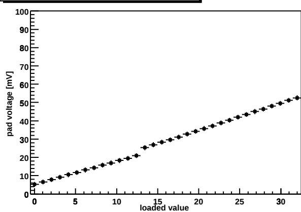
Chip Z36459A-W03-X09-Y04 shaper DAC
