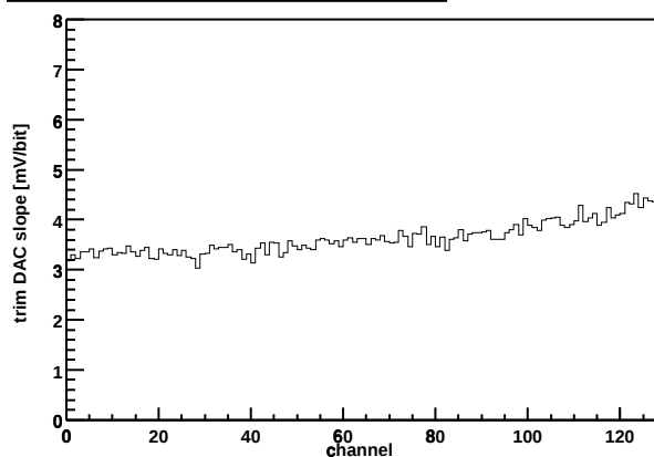
Chip Z36459A-W03-X09-Y04 Trim DAC slope vs. channel
