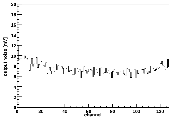
Chip Z36459A-W03-X09-Y04 Output noise vs. channel
