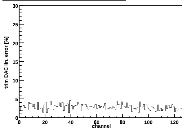
Chip Z36459A-W03-X09-Y04 trim DAC lin. error
