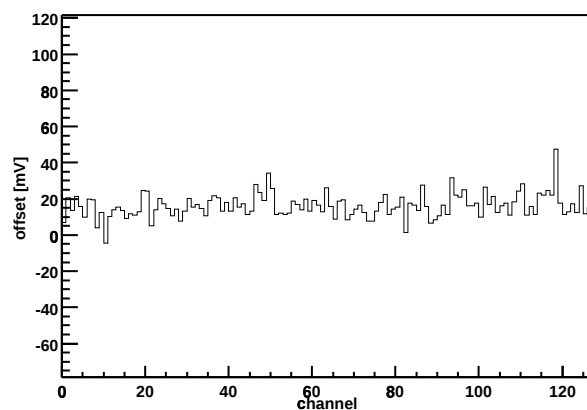
Chip Z36459A-W03-X09-Y04 Offset vs. channel
