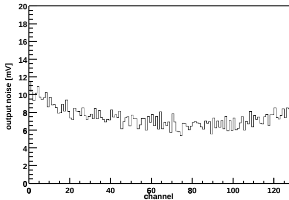
Chip Z36459A-W03-X09-Y05 Output noise vs. channel
