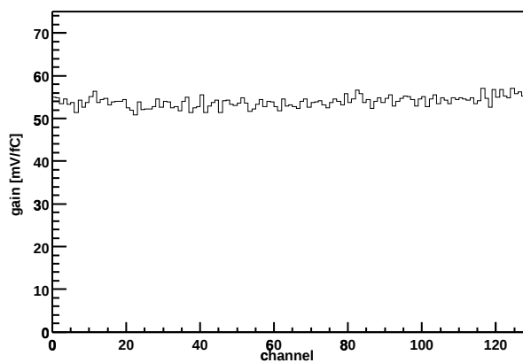
Chip Z36459A-W03-X09-Y05 Gain vs. channel
