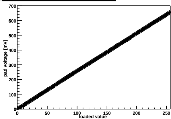
Chip Z36459A-W03-X09-Y05 threshold DAC
