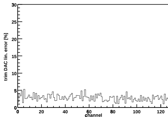
Chip Z36459A-W03-X09-Y05 trim DAC lin. error
