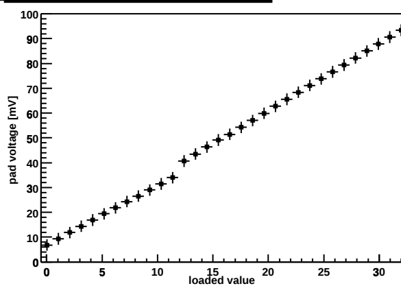
Chip Z36459A-W03-X09-Y05 preamp DAC
