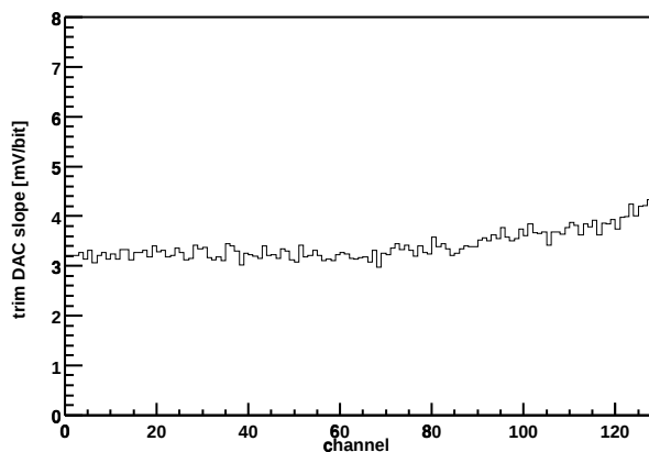
Chip Z36459A-W03-X09-Y05 Trim DAC slope vs. channel
