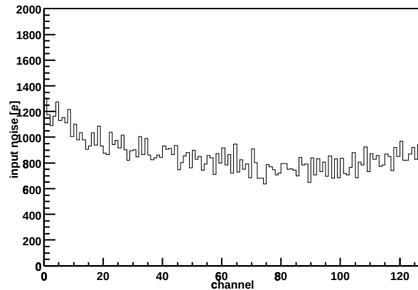
Chip Z36459A-W03-X09-Y05 Input noise vs. channel
