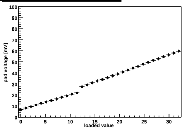
Chip Z36459A-W03-X09-Y05 shaper DAC
