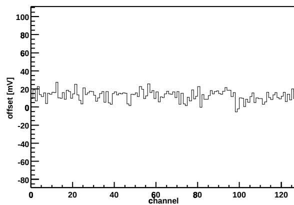
Chip Z36459A-W03-X09-Y05 Offset vs. channel
