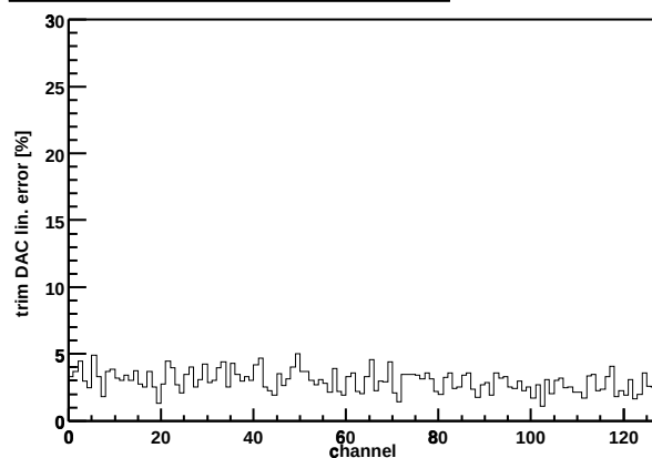
Chip Z36459A-W03-X09-Y11 trim DAC lin. error
