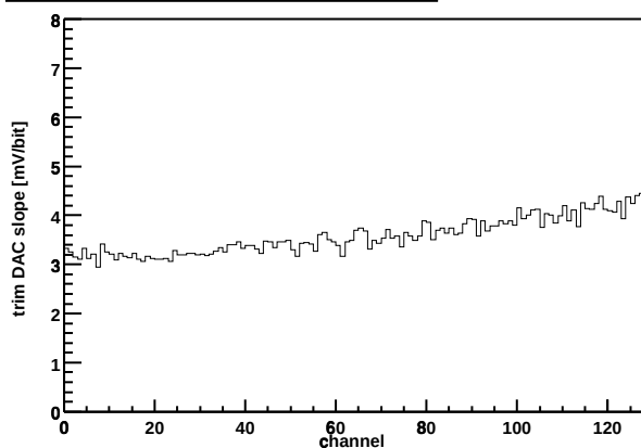
Chip Z36459A-W03-X09-Y11 Trim DAC slope vs. channel
