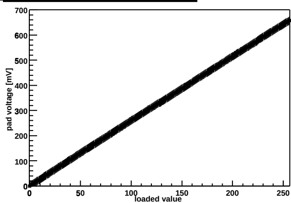
Chip Z36459A-W03-X09-Y11 threshold DAC
