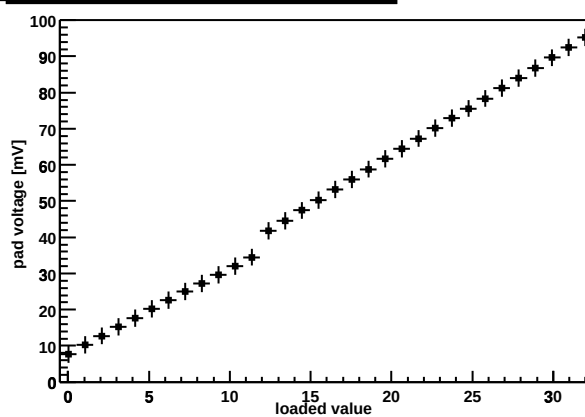
Chip Z36459A-W03-X09-Y11 preamp DAC
