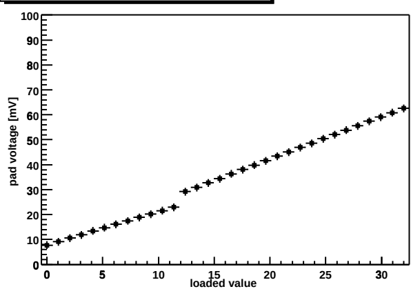
Chip Z36459A-W03-X09-Y11 shaper DAC
