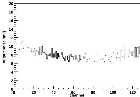
Chip Z36459A-W03-X09-Y11 Output noise vs. channel
