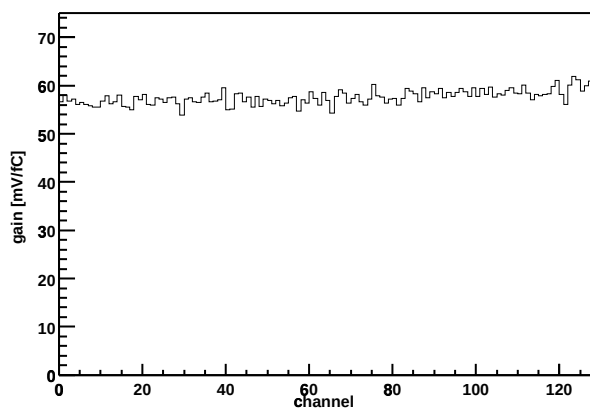
Chip Z36459A-W03-X09-Y11 Gain vs. channel
