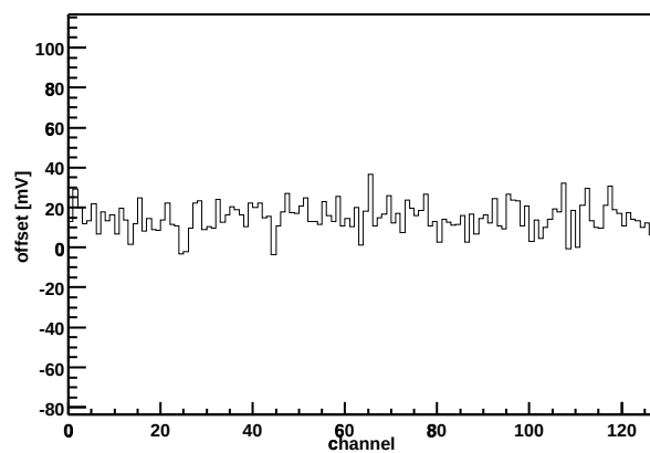
Chip Z36459A-W03-X09-Y11 Offset vs. channel
