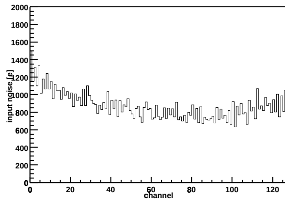
Chip Z36459A-W03-X09-Y11 Input noise vs. channel
