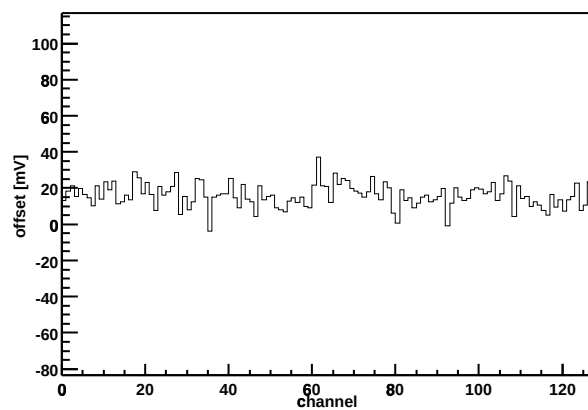
Chip Z36459A-W03-X09-Y16 Offset vs. channel
