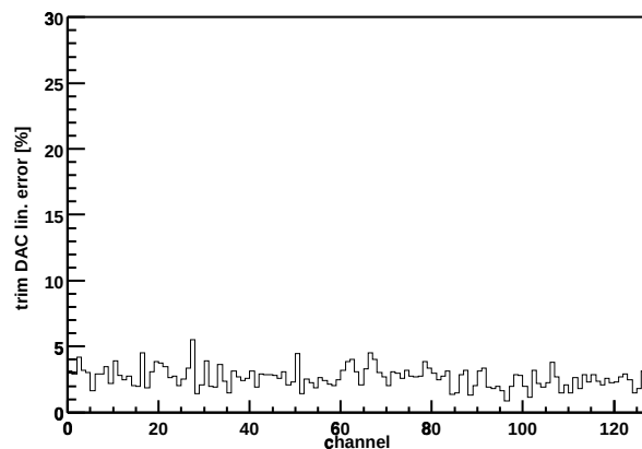
Chip Z36459A-W03-X09-Y16 trim DAC lin. error
