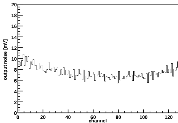
Chip Z36459A-W03-X09-Y16 Output noise vs. channel
