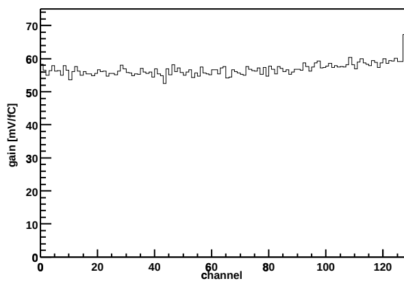
Chip Z36459A-W03-X09-Y16 Gain vs. channel
