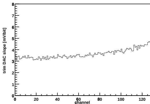
Chip Z36459A-W03-X09-Y16 Trim DAC slope vs. channel
