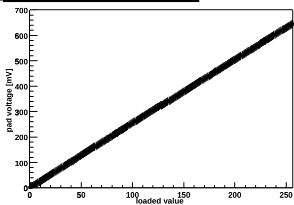
Chip Z36459A-W03-X09-Y16 threshold DAC
