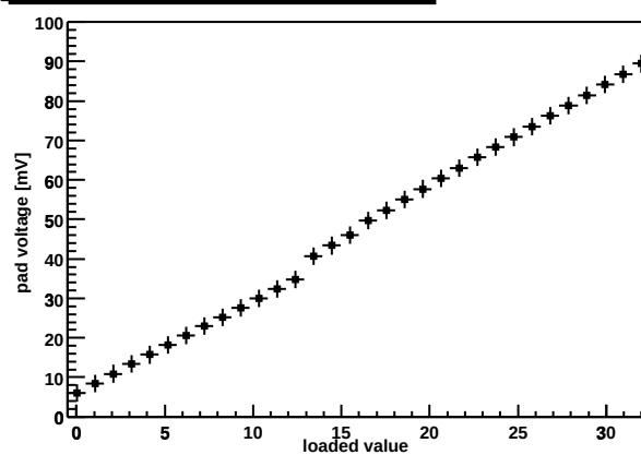
Chip Z36459A-W03-X09-Y16 preamp DAC
