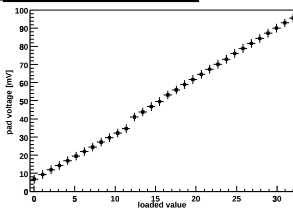
Chip Z36459A-W03-X09-Y19 preamp DAC
