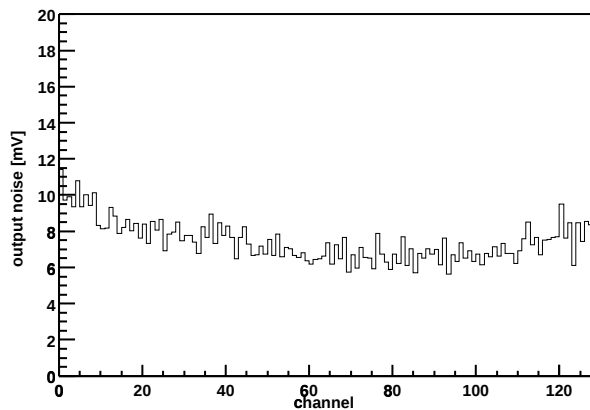
Chip Z36459A-W03-X09-Y19 Output noise vs. channel
