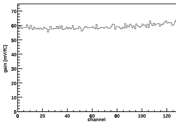
Chip Z36459A-W03-X09-Y19 Gain vs. channel
