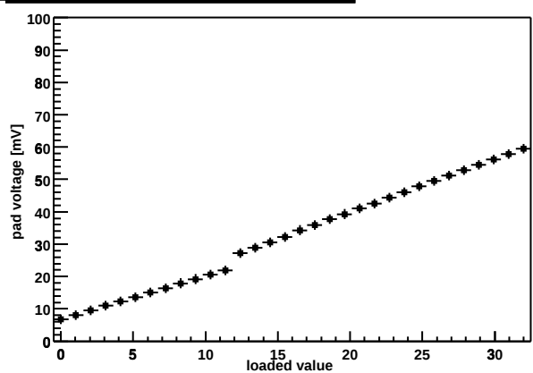
Chip Z36459A-W03-X09-Y19 shaper DAC
