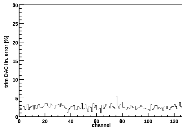
Chip Z36459A-W03-X09-Y19 trim DAC lin. error
