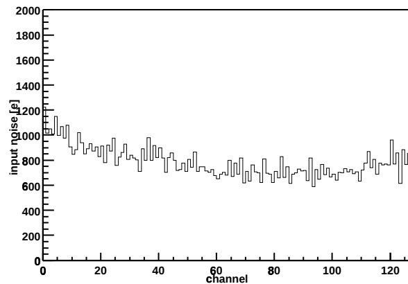
Chip Z36459A-W03-X09-Y19 Input noise vs. channel
