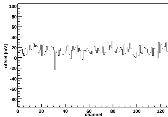
Chip Z36459A-W03-X09-Y19 Offset vs. channel
