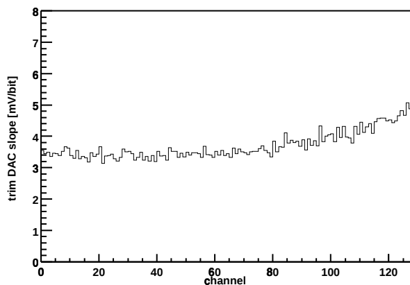
Chip Z36459A-W03-X09-Y19 Trim DAC slope vs. channel
