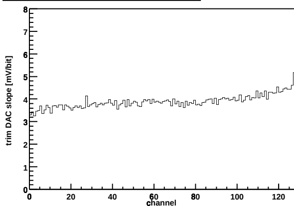
Chip Z36459A-W03-X10-Y00 Trim DAC slope vs. channel
