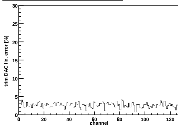
Chip Z36459A-W03-X10-Y00 trim DAC lin. error
