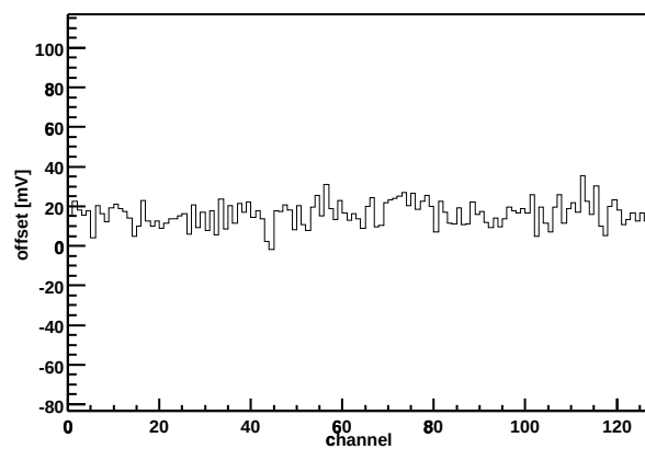
Chip Z36459A-W03-X10-Y00 Offset vs. channel
