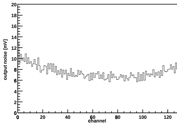
Chip Z36459A-W03-X10-Y00 Output noise vs. channel
