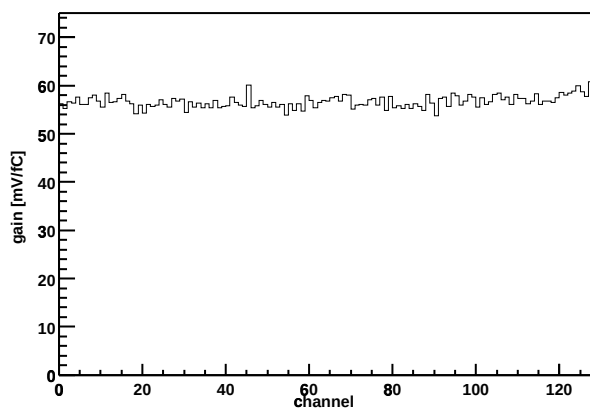
Chip Z36459A-W03-X10-Y00 Gain vs. channel
