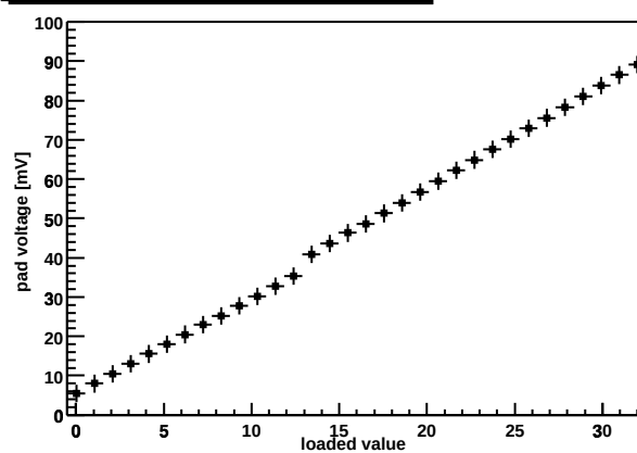
Chip Z36459A-W03-X10-Y00 preamp DAC
