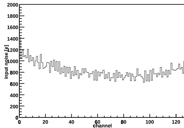
Chip Z36459A-W03-X10-Y00 Input noise vs. channel
