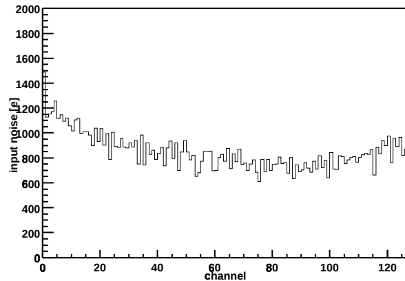
Chip Z36459A-W03-X10-Y03 Input noise vs. channel
