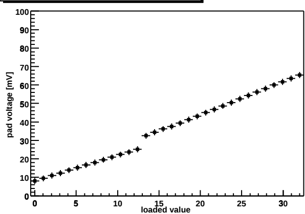
Chip Z36459A-W03-X10-Y03 shaper DAC
