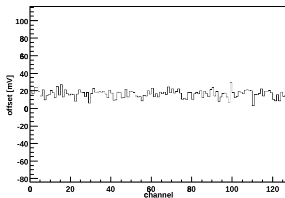
Chip Z36459A-W03-X10-Y03 Offset vs. channel
