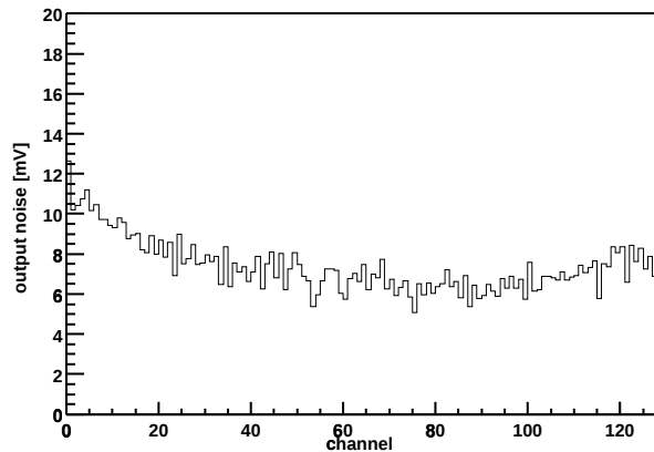
Chip Z36459A-W03-X10-Y03 Output noise vs. channel
