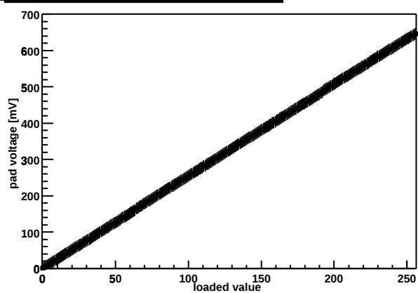
Chip Z36459A-W03-X10-Y03 threshold DAC
