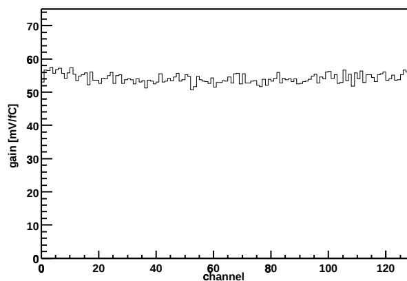
Chip Z36459A-W03-X10-Y03 Gain vs. channel
