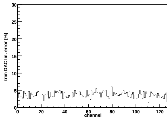
Chip Z36459A-W03-X10-Y03 trim DAC lin. error
