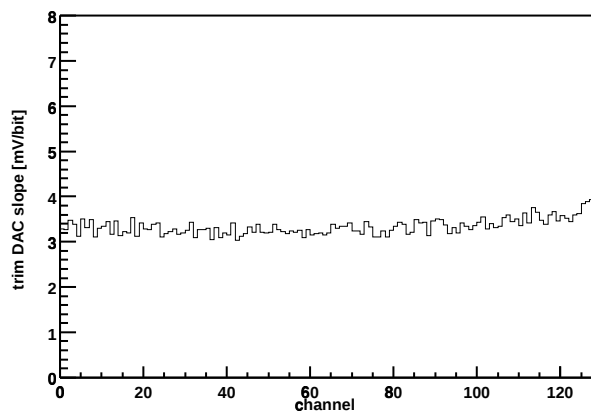
Chip Z36459A-W03-X10-Y03 Trim DAC slope vs. channel
