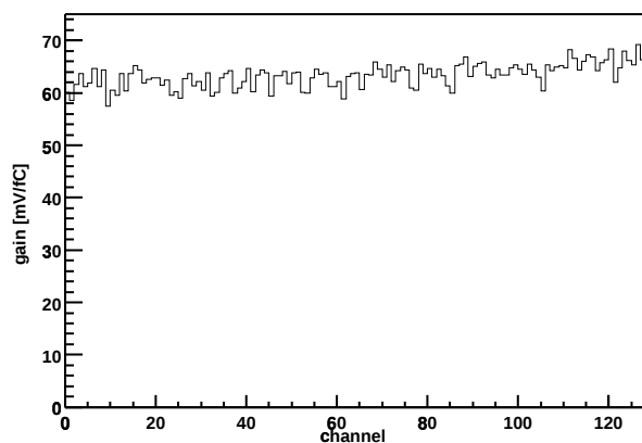
Chip Z36459A-W03-X10-Y06 Gain vs. channel
