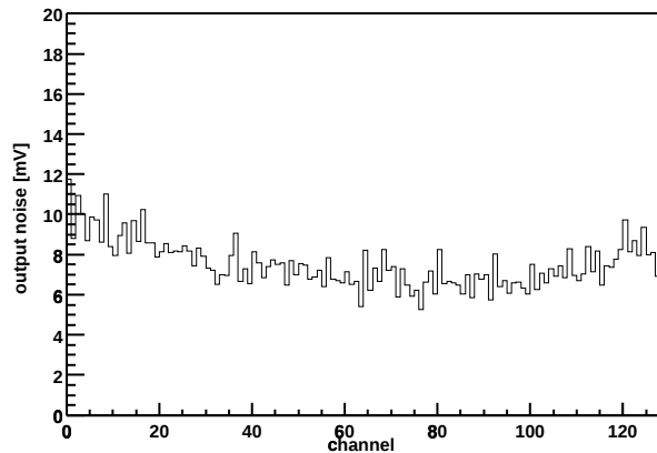
Chip Z36459A-W03-X10-Y06 Output noise vs. channel
