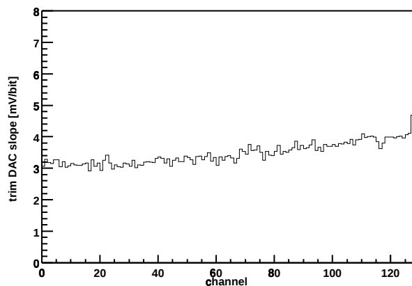
Chip Z36459A-W03-X10-Y06 Trim DAC slope vs. channel
