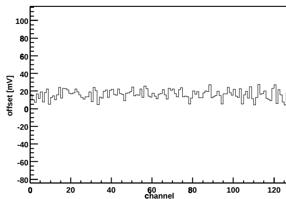
Chip Z36459A-W03-X10-Y06 Offset vs. channel
