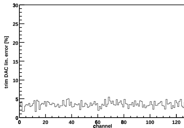
Chip Z36459A-W03-X10-Y06 trim DAC lin. error
