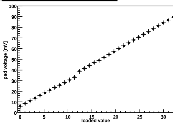
Chip Z36459A-W03-X10-Y06 preamp DAC
