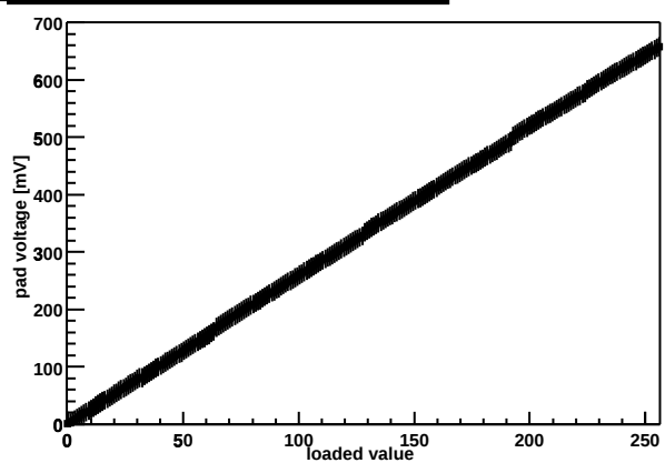
Chip Z36459A-W03-X10-Y06 threshold DAC
