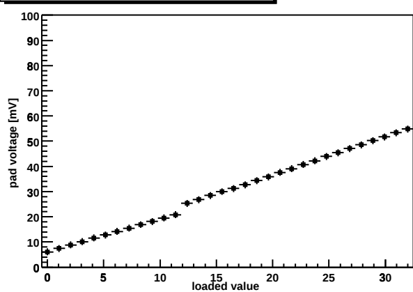
Chip Z36459A-W03-X10-Y06 shaper DAC
