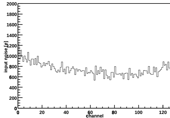
Chip Z36459A-W03-X10-Y06 Input noise vs. channel
