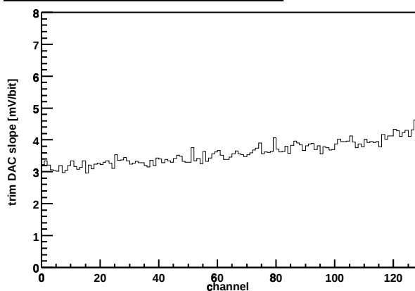
Chip Z36459A-W03-X10-Y09 Trim DAC slope vs. channel
