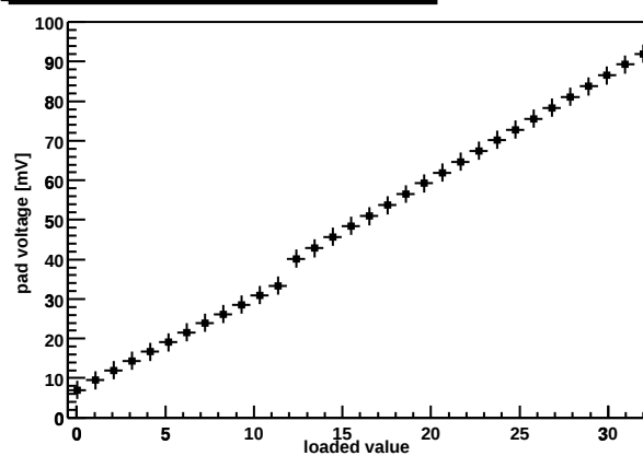
Chip Z36459A-W03-X10-Y09 preamp DAC
