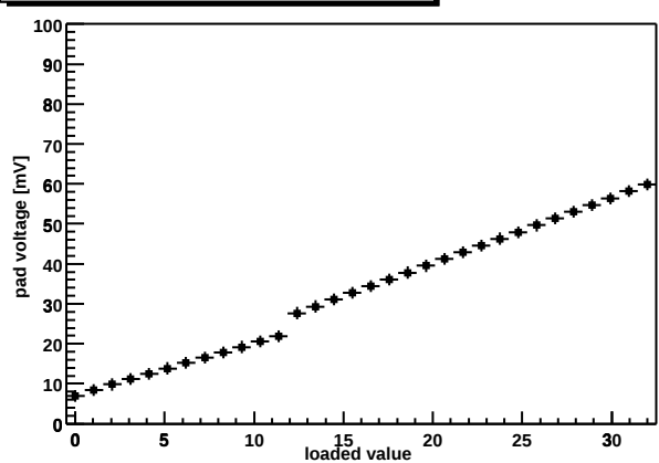
Chip Z36459A-W03-X10-Y09 shaper DAC
