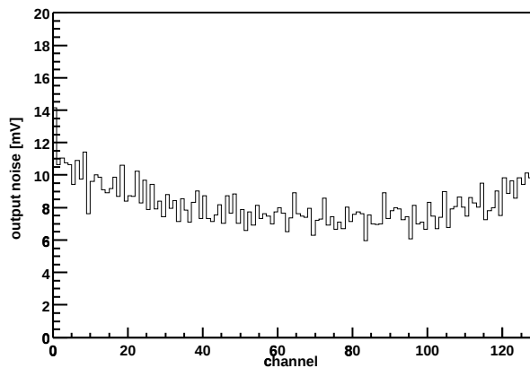
Chip Z36459A-W03-X10-Y09 Output noise vs. channel
