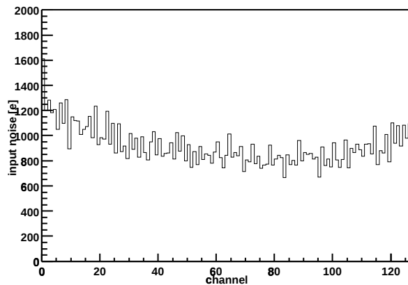
Chip Z36459A-W03-X10-Y09 Input noise vs. channel
