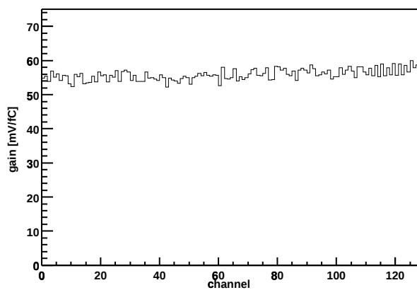
Chip Z36459A-W03-X10-Y09 Gain vs. channel
