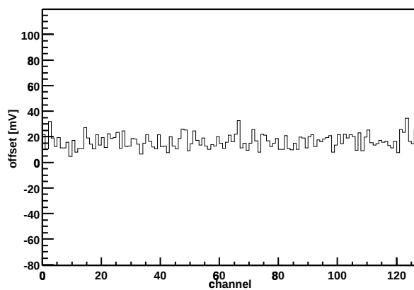
Chip Z36459A-W03-X10-Y09 Offset vs. channel
