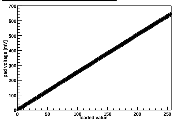
Chip Z36459A-W03-X10-Y09 threshold DAC
