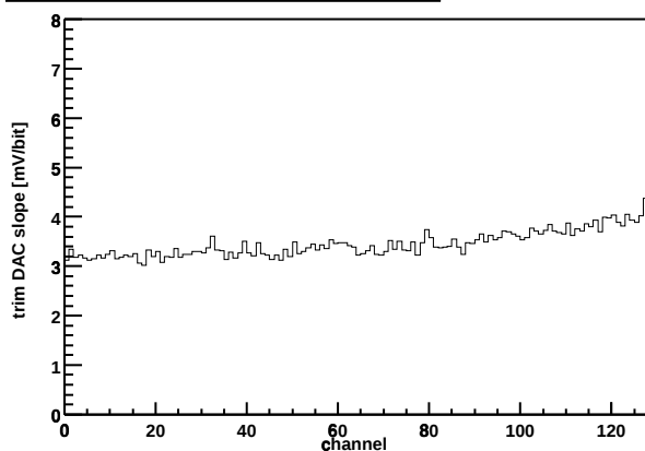
Chip Z36459A-W03-X10-Y10 Trim DAC slope vs. channel
