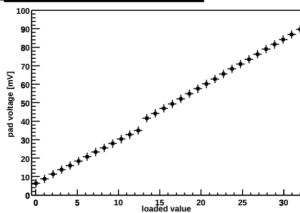
Chip Z36459A-W03-X10-Y10 preamp DAC
