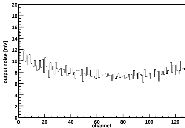
Chip Z36459A-W03-X10-Y10 Output noise vs. channel
