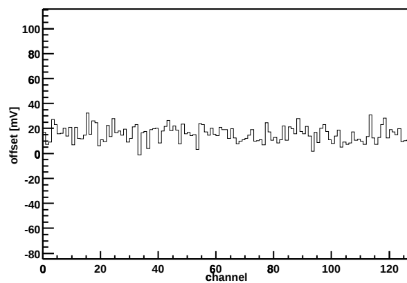
Chip Z36459A-W03-X10-Y10 Offset vs. channel
