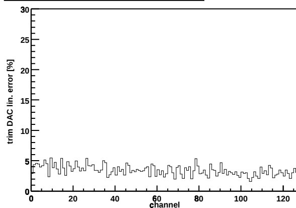
Chip Z36459A-W03-X10-Y10 trim DAC lin. error
