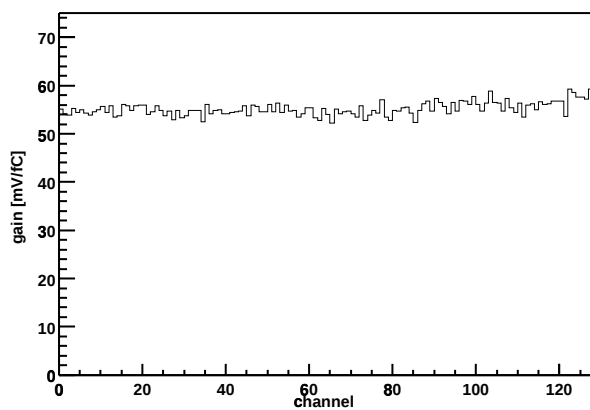
Chip Z36459A-W03-X10-Y10 Gain vs. channel
