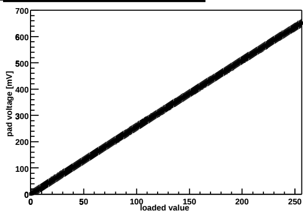
Chip Z36459A-W03-X10-Y10 threshold DAC
