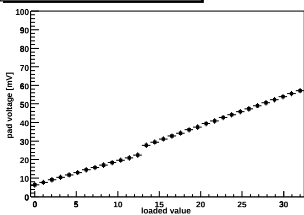
Chip Z36459A-W03-X10-Y10 shaper DAC
