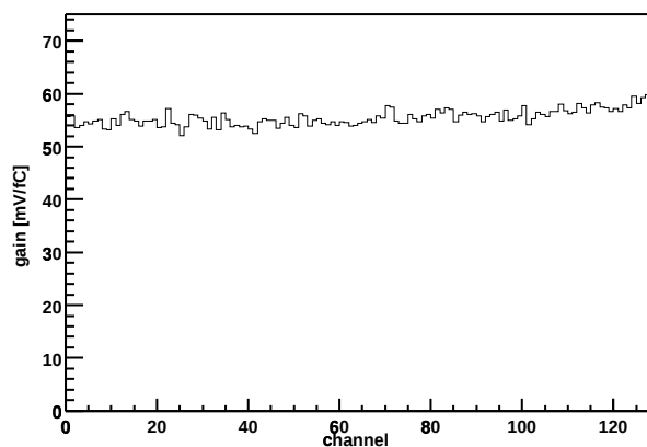
Chip Z36459A-W03-X10-Y16 Gain vs. channel
