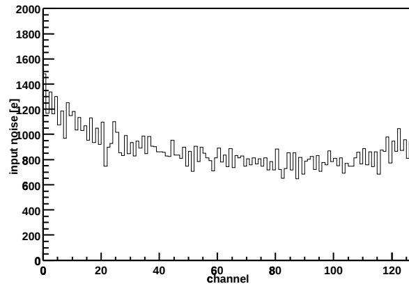
Chip Z36459A-W03-X10-Y16 Input noise vs. channel
