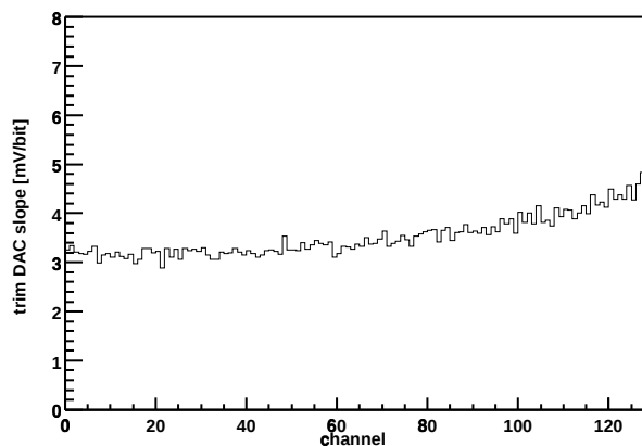
Chip Z36459A-W03-X10-Y16 Trim DAC slope vs. channel
