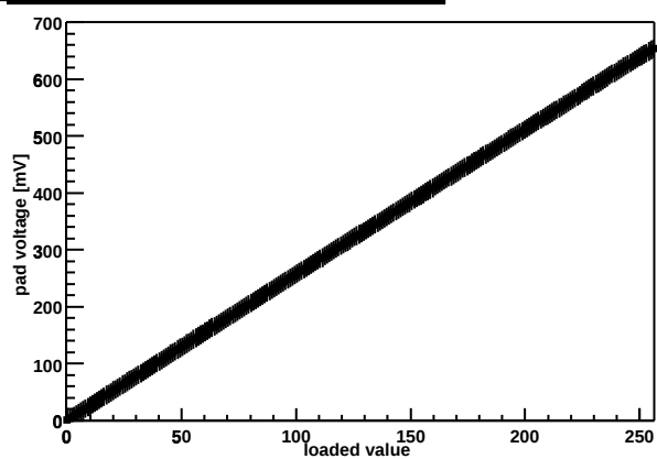
Chip Z36459A-W03-X10-Y16 threshold DAC
