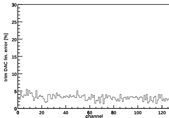
Chip Z36459A-W03-X10-Y16 trim DAC lin. error
