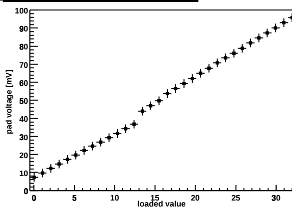
Chip Z36459A-W03-X10-Y16 preamp DAC
