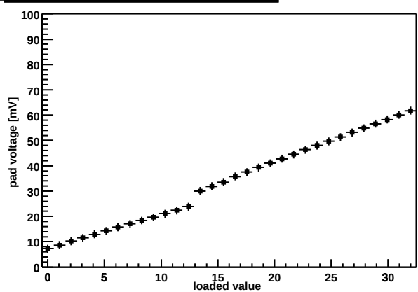
Chip Z36459A-W03-X10-Y16 shaper DAC
