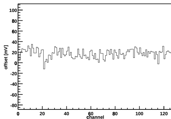
Chip Z36459A-W03-X10-Y16 Offset vs. channel
