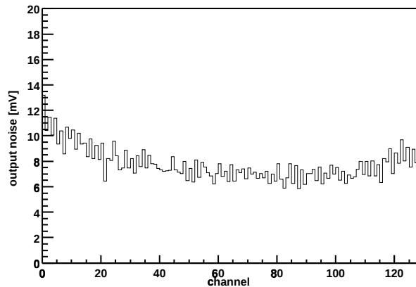
Chip Z36459A-W03-X10-Y16 Output noise vs. channel
