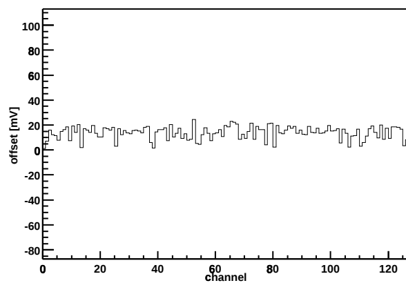
Chip Z36459A-W03-X11-Y02 Offset vs. channel
