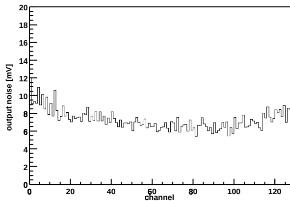
Chip Z36459A-W03-X11-Y02 Output noise vs. channel
