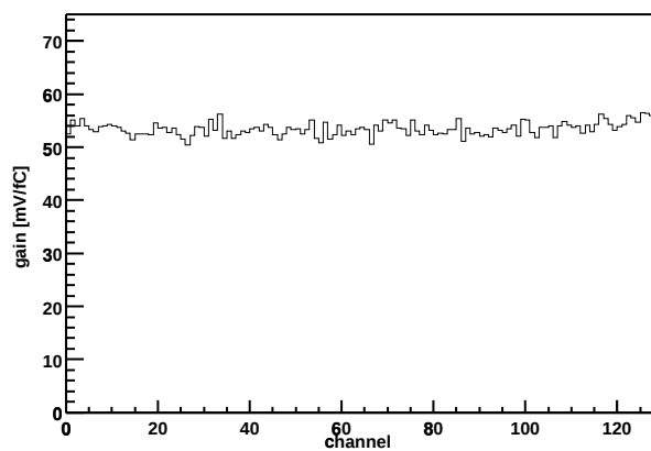
Chip Z36459A-W03-X11-Y02 Gain vs. channel
