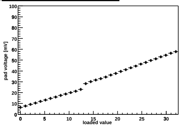
Chip Z36459A-W03-X11-Y02 shaper DAC
