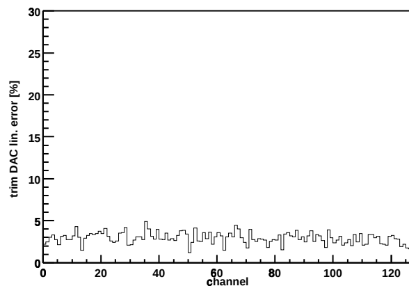
Chip Z36459A-W03-X11-Y02 trim DAC lin. error
