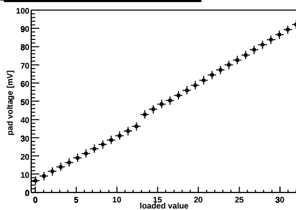
Chip Z36459A-W03-X11-Y02 preamp DAC
