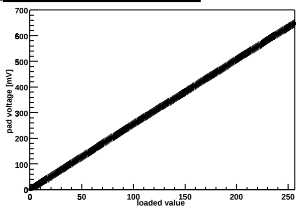
Chip Z36459A-W03-X11-Y02 threshold DAC
