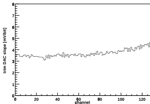
Chip Z36459A-W03-X11-Y02 Trim DAC slope vs. channel
