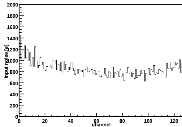
Chip Z36459A-W03-X11-Y02 Input noise vs. channel
