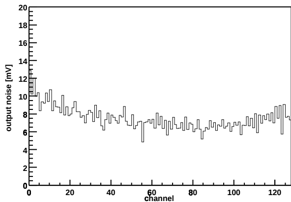
Chip Z36459A-W03-X11-Y03 Output noise vs. channel
