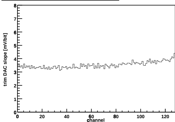
Chip Z36459A-W03-X11-Y03 Trim DAC slope vs. channel
