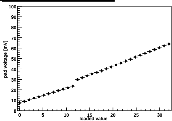
Chip Z36459A-W03-X11-Y03 shaper DAC
