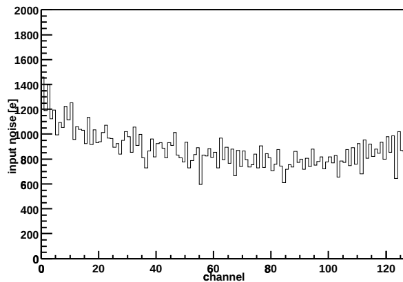
Chip Z36459A-W03-X11-Y03 Input noise vs. channel
