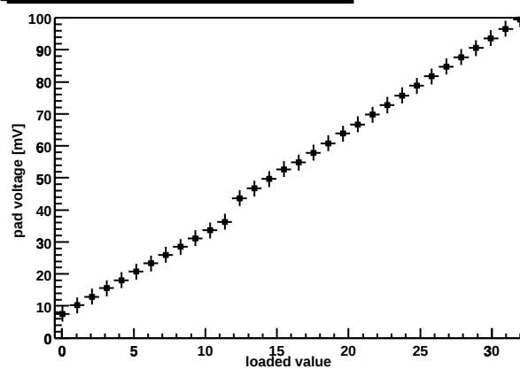
Chip Z36459A-W03-X11-Y03 preamp DAC
