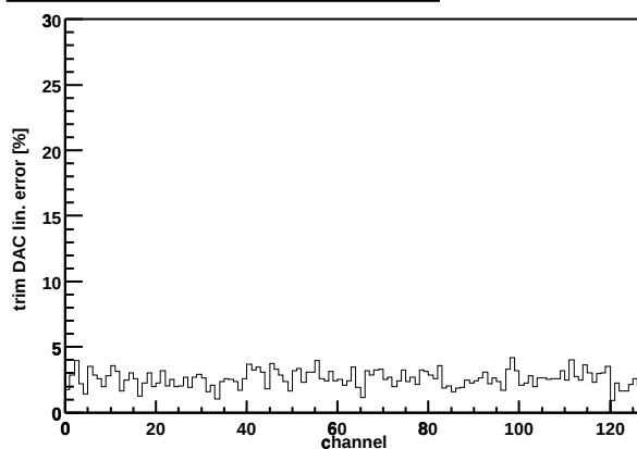
Chip Z36459A-W03-X11-Y03 trim DAC lin. error
