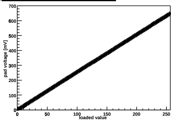
Chip Z36459A-W03-X11-Y03 threshold DAC
