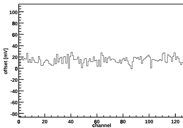
Chip Z36459A-W03-X11-Y03 Offset vs. channel
