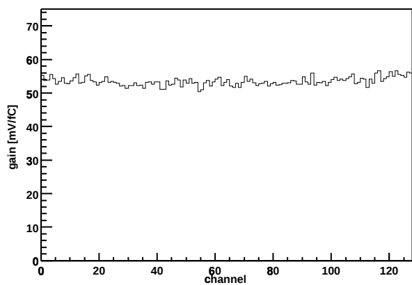
Chip Z36459A-W03-X11-Y03 Gain vs. channel
