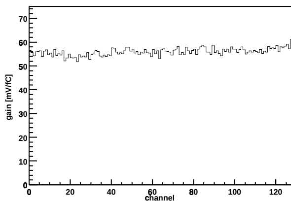
Chip Z36459A-W03-X11-Y08 Gain vs. channel
