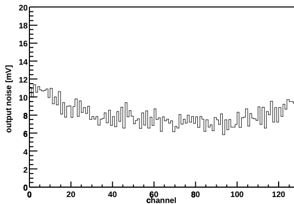
Chip Z36459A-W03-X11-Y08 Output noise vs. channel
