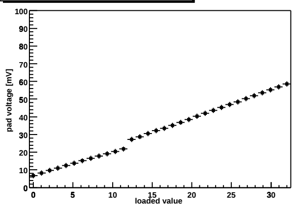
Chip Z36459A-W03-X11-Y08 shaper DAC
