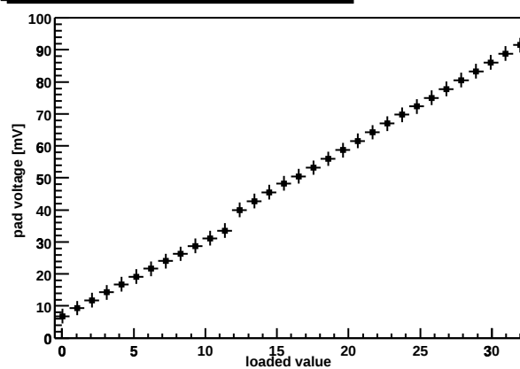
Chip Z36459A-W03-X11-Y08 preamp DAC
