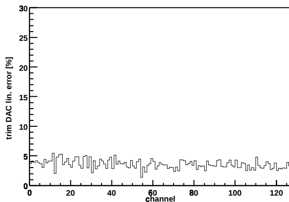
Chip Z36459A-W03-X11-Y08 trim DAC lin. error
