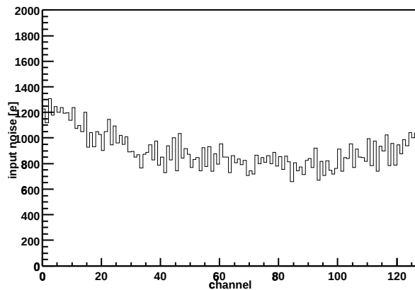
Chip Z36459A-W03-X11-Y08 Input noise vs. channel
