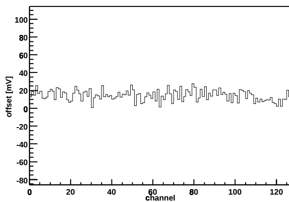
Chip Z36459A-W03-X11-Y08 Offset vs. channel
