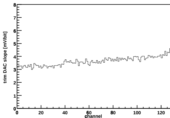
Chip Z36459A-W03-X11-Y08 Trim DAC slope vs. channel
