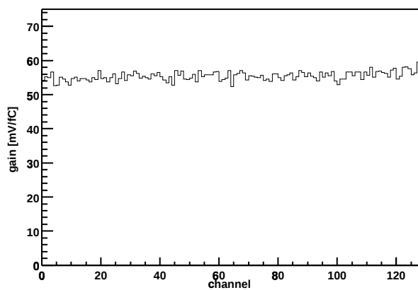
Chip Z36459A-W03-X11-Y09 Gain vs. channel
