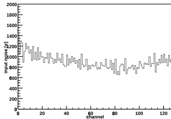
Chip Z36459A-W03-X11-Y09 Input noise vs. channel
