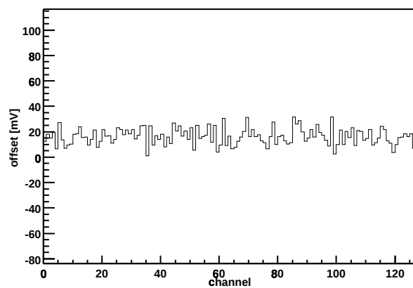
Chip Z36459A-W03-X11-Y09 Offset vs. channel
