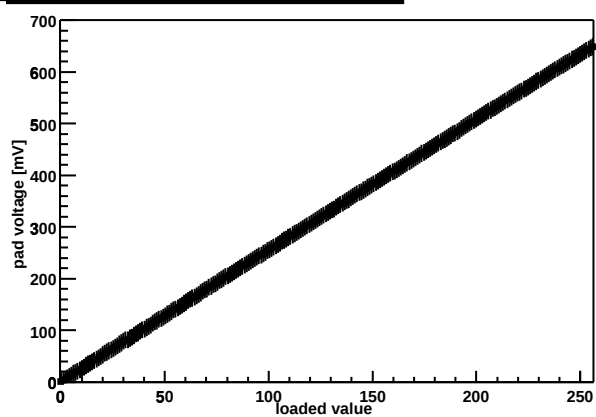
Chip Z36459A-W03-X11-Y09 threshold DAC
