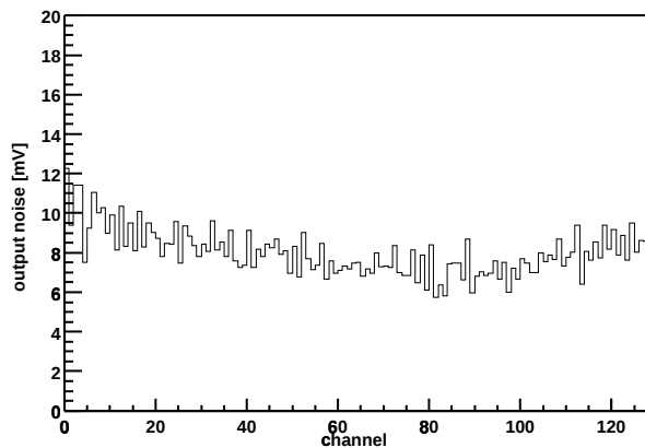
Chip Z36459A-W03-X11-Y09 Output noise vs. channel
