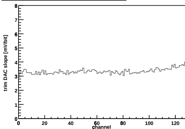
Chip Z36459A-W03-X11-Y09 Trim DAC slope vs. channel
