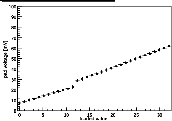
Chip Z36459A-W03-X11-Y09 shaper DAC
